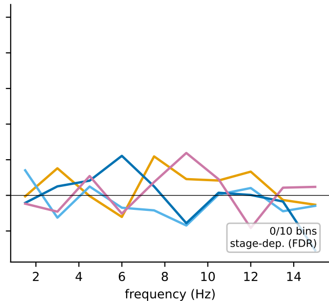
B between-channel (Fpz-Cz ↔ Pz-Oz) IAAFT null
