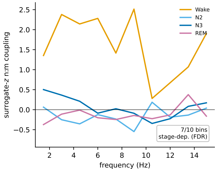
A within-channel (Fpz-Cz) waveform-preserving (time-shuffle) null
