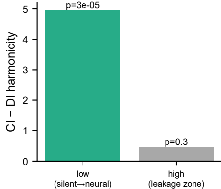
B Effect is in the silent band (neural, not leakage)
