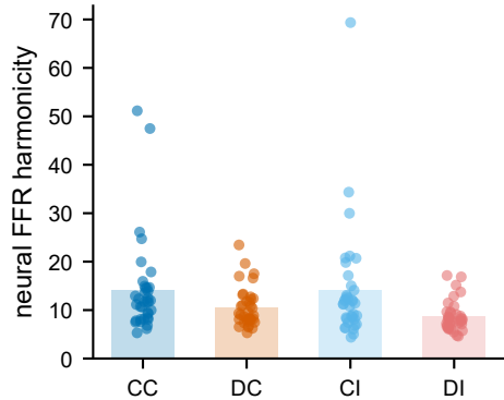
A Consonant > dissonant (incl. missing-fundamental)
