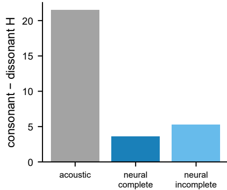
C Neural effect beyond acoustic leakage
