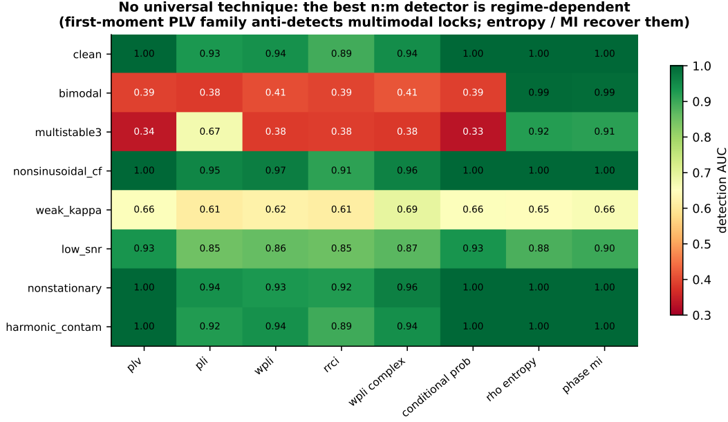
Figure 5: Complementary techniques across regimes. Detection AUC for eight techniques (columns) across eight coupling regimes (rows). The first-moment PLV family (left) is supreme on unimodal-style regimes but anti-detects the multimodal ones ( bimodal , multistable3 ), where the all-moment entropy and mutual-information indices (right) dominate.
