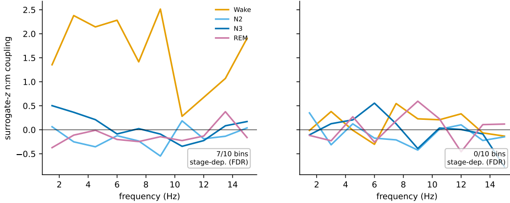
Stage-dependent n:m phase coupling is genuine within-channel (delta) but absent between channels (entropy; Sleep-EDF; whole-spectrum, surrogate-controlled) A within-channel (Fpz-Cz) waveform-preserving (time-shuffle) null B between-channel (Fpz-Cz ↔ Pz-Oz) IAAFT null
