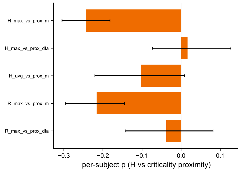
A. Is H higher near criticality? ( \rho > 0 = yes)
