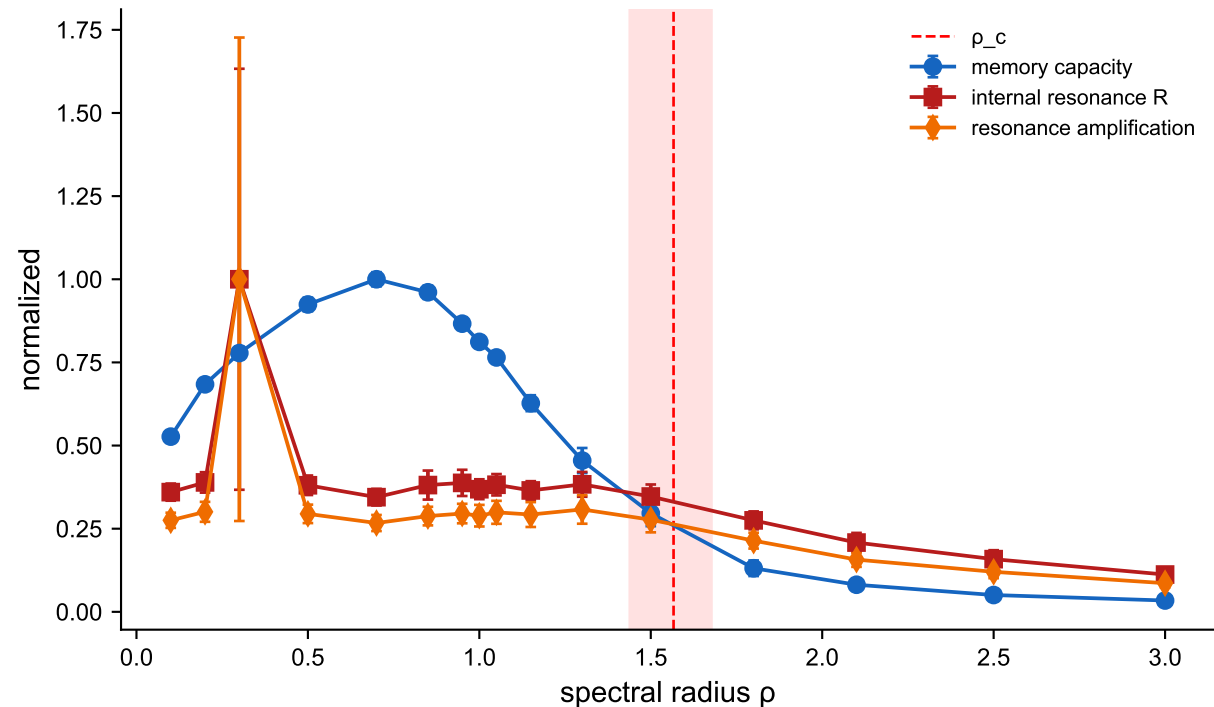
B. Resonance vs computation vs criticality MC & R peak in the ordered regime, below \rho_c (n=16 seeds)
