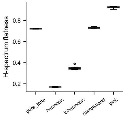
A H-flatness separates classes (harmonic 0.17 \rightarrow noise 0.92)
