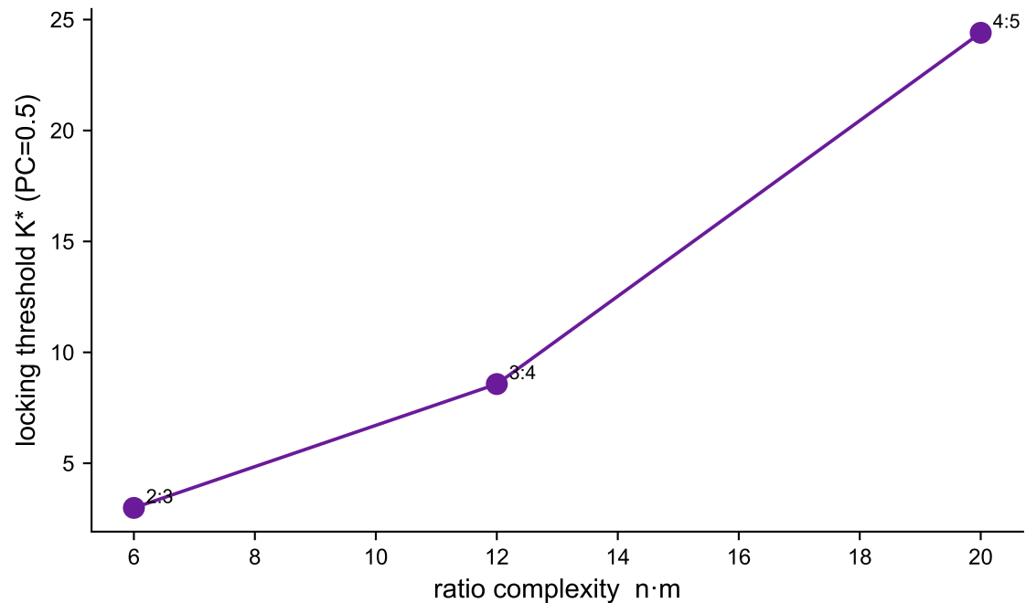
B. Threshold rises with complexity ( \rho = +1.00 )
