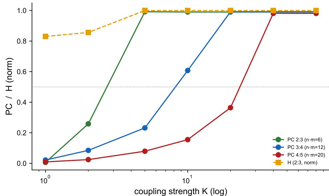
A. Complex ratios lock LATER (H flat: blind to coupling)
