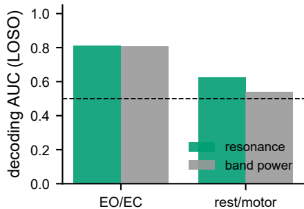
A EEG state decoding (LOSO AUC) (EO/EC \approx band power)
