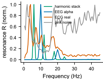
C Cross-modality (acc=0.99, chance 0.14)
