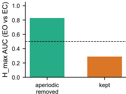
B 1/f confound control
