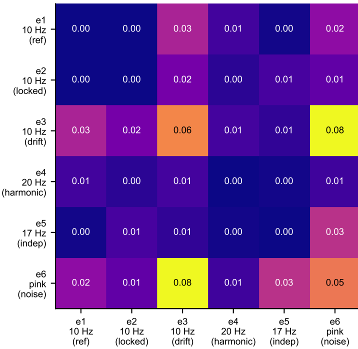
R = combine(harmmean)(H, PC)
