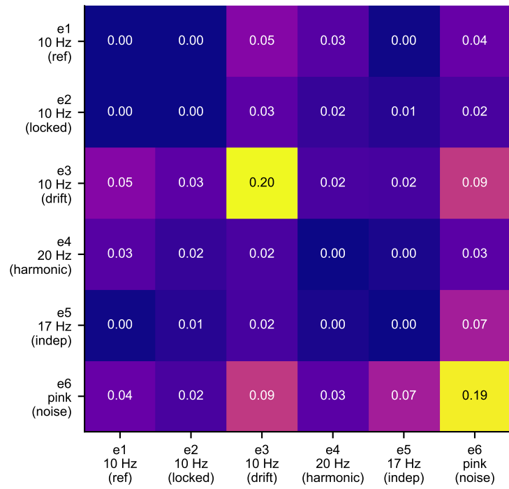
R = combine(min)(H, PC)
