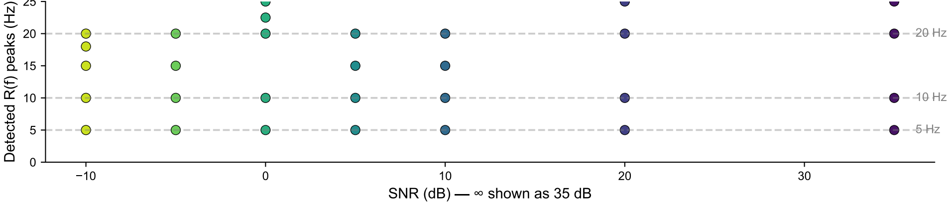
d) Detected peak frequencies vs SNR — true carriers at 5/10/20 Hz (grey lines)
