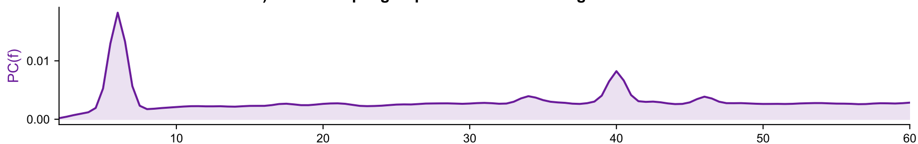
c) Phase coupling — peaks at theta and at gamma sidebands
