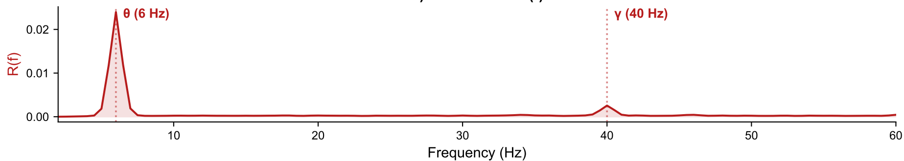
d) Resonance R(f)
