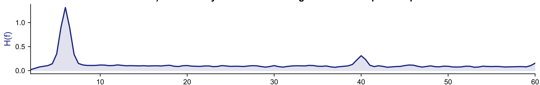
b) Harmonicity — both theta and gamma carriers picked up
