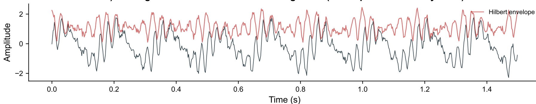
b) Harmonicity — both theta and gamma carriers picked up
