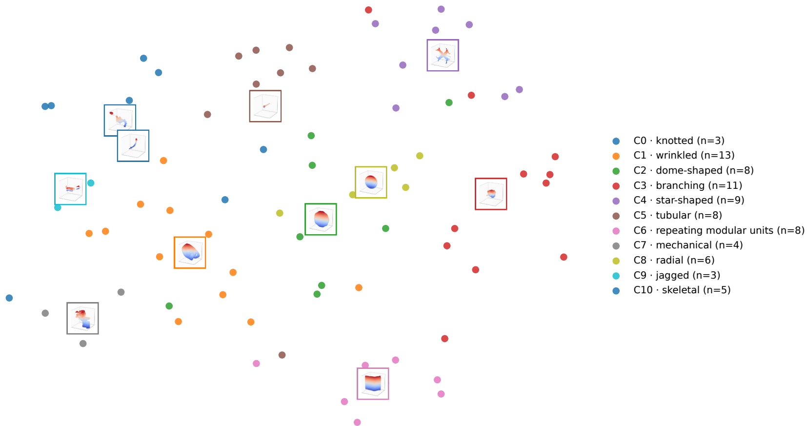
Families of dream-forms — OpenShape embeddings (t-SNE), 11 clusters
