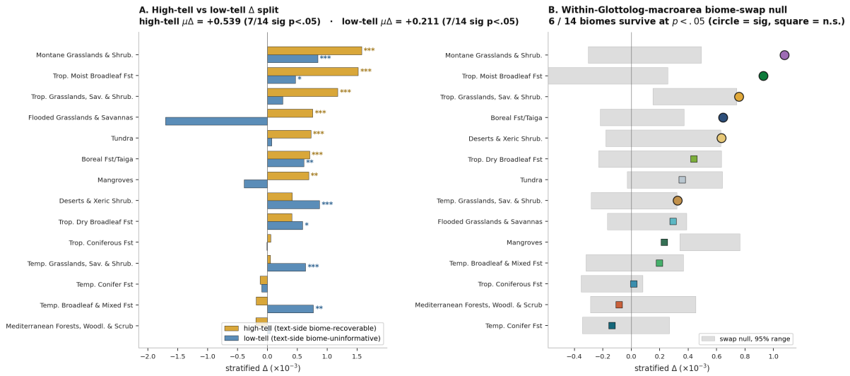
Figure 14. Biome-tell tests. Panel A: per-biome within-iconic-taxon stratified \Delta on the high-tell half (motifs whose anonymised text is biome-recoverable above chance, gold bars) and the low-tell half (motifs whose text alone is biome-uninformative, blue bars), across the 14 WWF biomes. Both halves carry positive across-biome mean \Delta ( +0.54 and +0.21 \times 10^{-3} respectively); seven biomes are individually significant at p < .05 in each half. Panel B: observed stratified \Delta per biome (coloured markers) overlaid on the 95% range of the within-Glottolog-macroarea biome-swap null distribution (grey strips). Circles mark biomes whose observed \Delta exceeds the 95th percentile of the swap null ( p < .05 ); squares mark biomes that do not. Six biomes survive this stricter null, indicating that biome content carries information beyond within-macro-area cultural autocorrelation.
