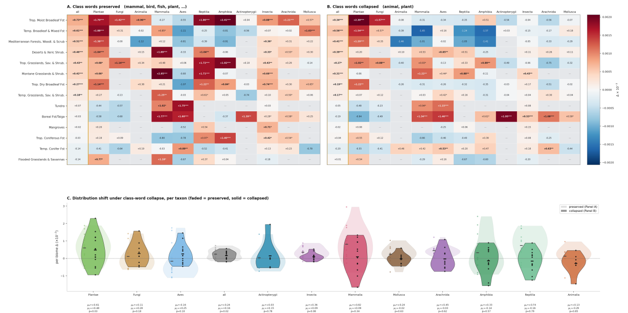
Figure 7. Per-taxon decomposition with class-word collapse control. Biome \times iconic-taxon residualised \Delta on sentence-pooled SigLIP-2 over the full LLM-clean corpus. Panel A : class words preserved – every specific species name has been replaced by its class word (mammal / bird / fish / tree / plant, etc.) but the class words remain distinct. Panel B : class words collapsed – every animal-kingdom class word further reduced to the single token animal and every plant-kingdom word to plant , so class-word frequency is identical across biomes by construction. Rows are the 14 WWF biomes, ordered by descending pooled (all) \Delta in Panel A. Cell values are per-biome per-taxon \Delta in \times 10^{-3} , with stars for nominal significance and bold for BH- q < 0.05 within the taxon. Cells with fewer than 10 biome-taxon photographs are shown as grey em-dashes. The gold-bordered all column anchors the marginal headline. Panel C : for each taxon, a double-violin contrasts the distribution of its 14 biome cells under the two encodings – faded behind for Panel A, solid in front for Panel B. Taxa are ordered left-to-right by descending collapsed mean \mu_C . Mean markers and per-taxon Wilcoxon p-values (against \Delta = 0 ) appear beneath. Plantae, Fungi, Aves, and Insecta retain most of their across-biome alignment under collapse, indicating that the per-(biome, taxon) coupling for those taxa is carried by surrounding lexical-thematic content (activities, landform vocabulary, narrative shape) rather than by the class word alone. Mammalia, Reptilia, and Amphibia attenuate substantially, indicating that a large part of their preserved- encoding signal was class-word frequency mirroring image-class frequency.
