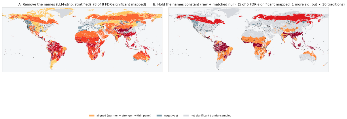
Figure 17. Same biome geography from two independent identity controls. Per-biome alignment on iNaturalist, mapped onto the WWF ecoregions. Panel A removes the names (LLM-strip within-iconic-taxon stratified \Delta , motif-to-biome permutation null); Panel B holds the names constant (raw myths, discrete matched-permutation null). Each panel paints only the biomes that reach Benjamini–Hochberg q < 0.05 with positive \Delta (8 of 14 and 6 of 14 respectively, five shared); one further matched-null biome (Mangroves) is significant but has fewer than ten traditions and is left grey. Warmer is stronger within each panel; the colour scales are per-panel and not comparable across panels. Black dots mark tradition centroids.
