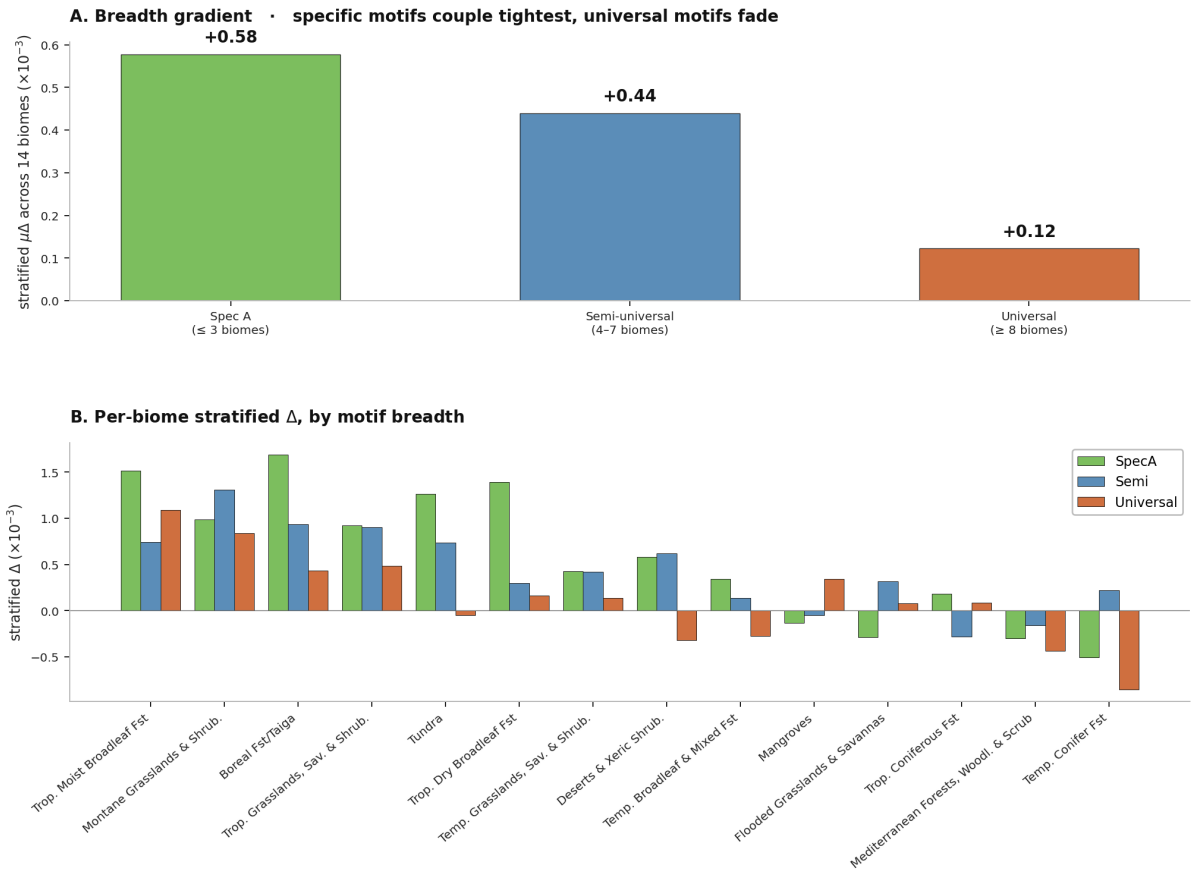
Figure 5. Breadth-stratified analysis. Panel A: across-biomes mean within-iconic-taxon stratified \Delta on iNaturalist, partitioned by motif breadth into three groups (Spec A: motifs touching \leq 3 biomes; semi-universal: 4–7 biomes; universal: \geq 8 biomes). The stratified \mu\Delta decays monotonically from +0.58 \times 10^{-3} (Spec A) through +0.44 \times 10^{-3} (semi-universal) to +0.12 \times 10^{-3} (universal); the marginal \Delta declines in parallel ( +0.52 \rightarrow +0.26 \rightarrow +0.05 \times 10^{-3} , reported in the text). This is the pattern most naturally expected if local ecological affordances contribute to motif stabilisation. Panel B: per-biome stratified \Delta within each breadth group, with biomes ordered by mean stratified \Delta across the three groups. Spec A bars (green) systematically dominate at the high- \Delta biomes (Tropical Moist Broadleaf, Boreal/Taiga, Tropical Grasslands, Tundra, Tropical Dry Broadleaf); universal bars (red) systematically lie at or below zero across most biomes.
