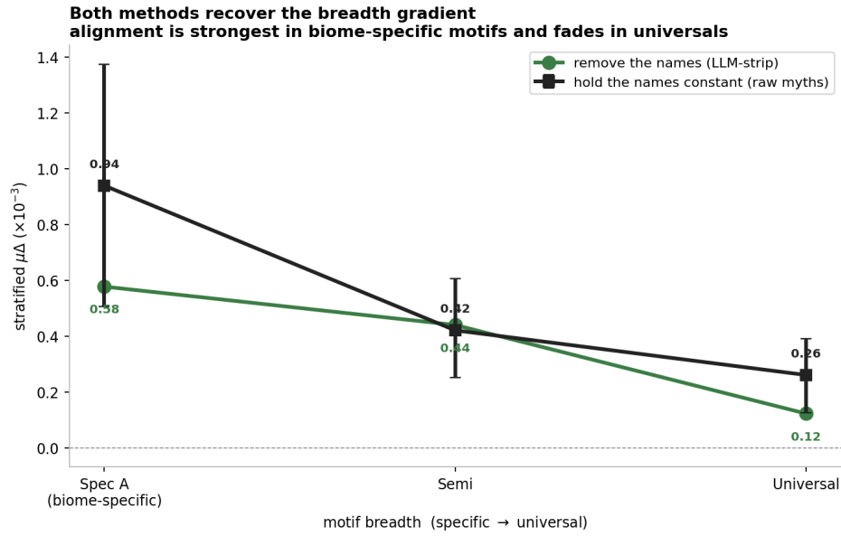
Figure 17. Both strategies recover the breadth gradient. Within-iconic-taxon stratified \mu\Delta on iNaturalist by motif breadth (biome-specific Spec A → semi-universal → universal), for the LLM-strip corpus (green) and the raw myths under the matched null (black, with 95% bootstrap CIs). Both decay monotonically from specific to universal motifs. The raw track sits higher in magnitude because identity content is still present in the un-anonymised embedding, but the shape of the gradient is shared.
