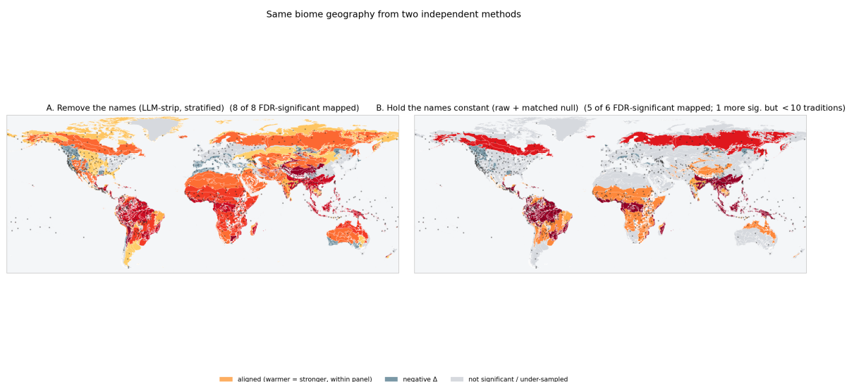
Figure 16. Same biome geography from two independent identity controls. Per-biome alignment on iNaturalist, mapped onto the WWF ecoregions. Panel A removes the names (LLM-strip within-iconic-taxon stratified \Delta , motif-to-biome permutation null); Panel B holds the names constant (raw myths, discrete matched-permutation null). Each panel paints only the biomes that reach Benjamini–Hochberg q < 0.05 with positive \Delta (8 of 14 and 6 of 14 respectively, five shared); one further matched-null biome (Mangroves) is significant but has fewer than ten traditions and is left grey. Warmer is stronger within each panel; the colour scales are per-panel and not comparable across panels. Black dots mark tradition centroids.
