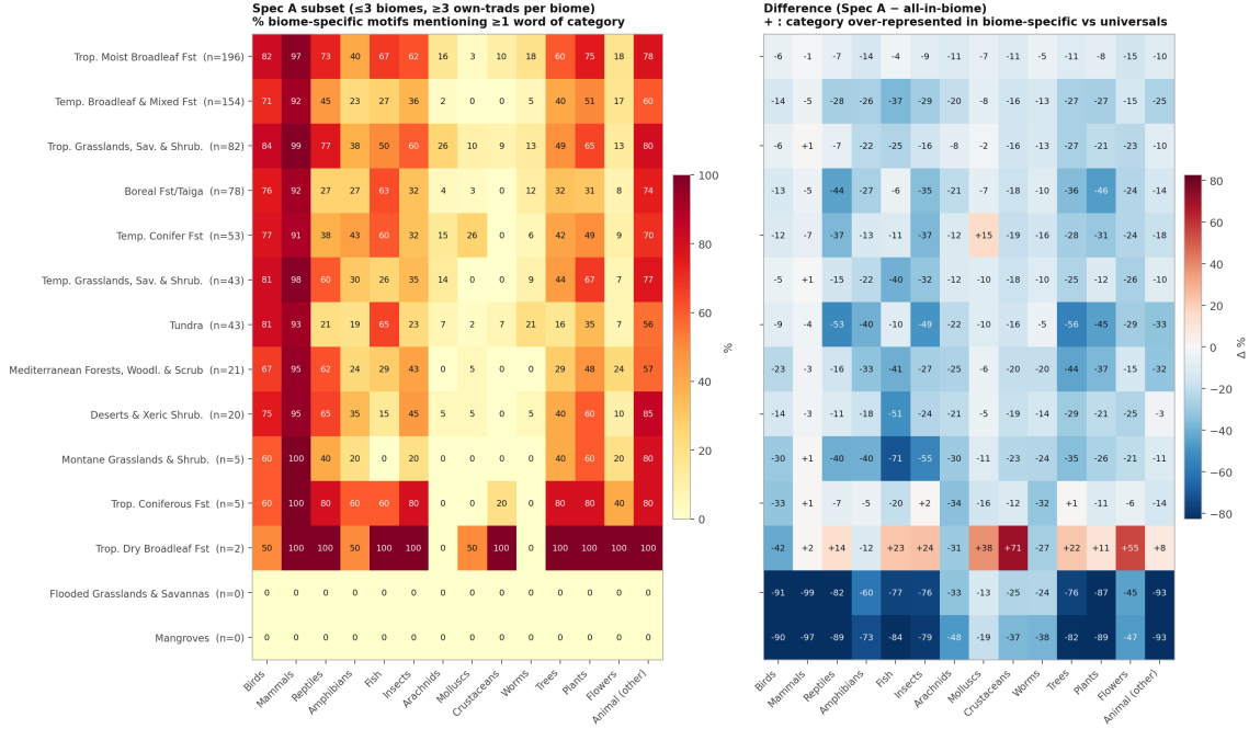
Figure 15. Ecological composition per biome (Spec A subset). Left: for each WWF biome (rows) and each of 14 taxonomic and botanical categories (columns), the cell shows the percentage of Spec A motifs (motifs touching \leq 3 biomes, as in the breadth analysis) with at least three of their traditions in that biome, whose raw Russian abstract mentions at least one species or plant of that category, before anonymisation. Right: difference (Spec A minus all-in-biome). Positive cells mark categories over-represented in biome-specific motifs relative to the universal-dominated full pool, revealing the ecological fingerprint that the species-hypernymisation layer subsequently removes. The all-motifs version of the heatmap is dominated by universal motifs and therefore uniformly red across biomes; we omit it here and release the underlying counts in the data drop.
