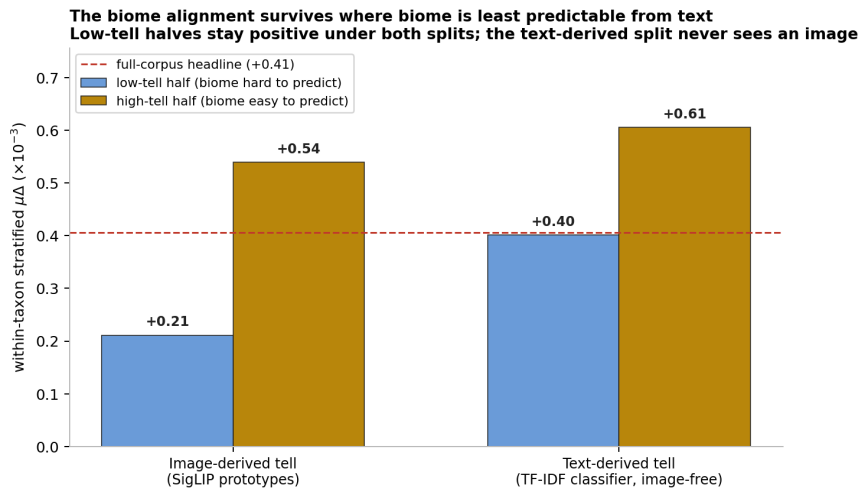
Figure 13. The biome alignment survives where biome is least predictable from the text alone. Within-iconic-taxon stratified \mu\Delta on the low- and high-tell halves under two median splits: the vision-model tell (SigLIP myth-to-image-prototype similarity) and a fully image-free text-only tell (an out-of-fold TF-IDF plus logistic-regression biome classifier). Both low-tell halves stay positive; the text-only low-tell half reaches the full-corpus headline (dashed line, +0.41 \times 10^{-3} ), so the alignment is not reducible to biome-correlated vocabulary a text model can exploit.
