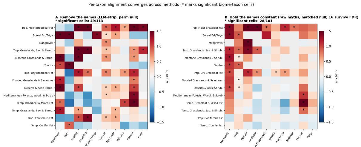
Figure 18. Per-taxon alignment converges across strategies. Per-(biome \times iconic-taxon) \Delta on iNaturalist. Panel A : remove the names (LLM-strip, motif-to-biome permutation null; 49 of 113 cells nominally significant). Panel B : hold the names constant (raw myths, matched null; 28 of 101 cells nominally significant, 16 surviving Benjamini–Hochberg FDR). Stars mark significant cells. The two matrices correlate at r = +0.64 , and the same vertebrate-and-plant taxa carry the signal under both controls.
