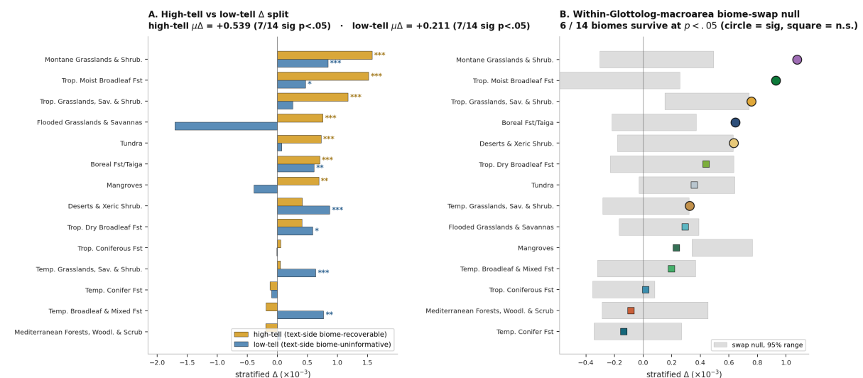
Figure 14. Biome-tell tests. Panel A: per-biome within-iconic-taxon stratified \Delta on the high-tell half (motifs whose anonymised text is biome-recoverable above chance, gold bars) and the low-tell half (motifs whose text alone is biome-uninformative, blue bars), across the 14 WWF biomes. Both halves carry positive across-biome mean \Delta ( +0.54 and +0.21 \times 10^{-3} respectively); seven biomes are individually significant at p < .05 in each half. Panel B: observed stratified \Delta per biome (coloured markers) overlaid on the 95% range of the within-Glottolog-macroarea biome-swap null distribution (grey strips). Circles mark biomes whose observed \Delta exceeds the 95th percentile of the swap null ( p < .05 ); squares mark biomes that do not. Six biomes survive this stricter null, indicating that biome content carries information beyond within-macro-area cultural autocorrelation.
