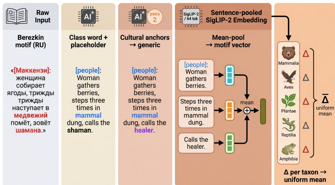
Figure 8. Pipeline schematic: anonymisation, sentence- pooled embedding, and image-side stratification. An example Berezkin motif (Mackenzie-region tradition, Boreal/Taiga) is threaded through the five stages of the analysis pipeline so the reader can trace one token’s journey from raw Russian to the final per-taxon \Delta . Stage 0 (Raw input) . The Russian motif from Berezkin’s catalogue, with biome-anchoring tokens highlighted in red (the species name “медвежий” bear, the cultural anchor “шамана” shaman, the ethnonym “Маккензи”). Stage 1 (Class word + placeholder) . An LLM pass translates the text into English and applies seven noun-targeted anonymisation rules; specific species names become their class word (bear \rightarrow mammal), ethnonyms become [people], biome words are dropped. Replaced tokens are shown in blue. Stage 2 (Cultural anchors \rightarrow generic) . A second LLM pass refines long-tail cultural anchors that survived Stage 1 (shaman \rightarrow healer, shown in purple); held-out audit on 200 random motifs confirms 96.5% strict-clean rate against species, place, and biome vocabulary. Stage 3 (Sentence-pooled SigLIP-2 embedding) . The cleaned abstract is split into sentences, each sentence is embedded independently within SigLIP-2’s 64-token window (mean 23 sentences per motif; 50,032 total across 2,158 motifs), and the per-motif vector is the mean-pooled, L2-renormalised sentence embedding. Stage 4 ( \Delta per taxon \rightarrow uniform mean) . On the image side, iNaturalist photographs of biome b are partitioned by iconic taxon (Mammalia, Aves, Plantae, Reptilia, Amphibia, ...). The motif vector’s residualised \Delta is computed within each taxon stratum and averaged uniformly across taxa, removing biome-by-taxon co-occurrence on the image side as a possible explanation of alignment.
