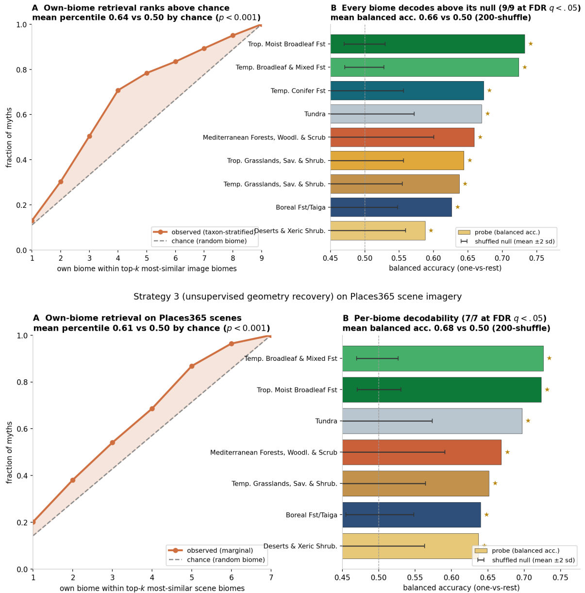
Figure 8. Biome structure is recoverable from the unsupervised myth-image affinity geometry, without using biome labels, on both image corpora. Each motif is represented by its residualised cosine-similarity profile across an image corpus; biome labels are never used to build the affinity geometry, and “own biome” is the biome contributing the most of a motif’s traditions. Top row, iNaturalist (46,481 species photographs). (A) Own-biome retrieval: the nine well-sampled biomes are ranked by each motif’s taxon-stratified mean similarity to their images; the curve gives the fraction of motifs whose own biome falls within the top k ranks (orange) against the chance diagonal (grey). Own biome reaches the 64th percentile on average ( p < .001 , 2,000 permutations). (B) Per-biome decodability: balanced accuracy of a five-fold one-versus-rest logistic probe on the PCA-50 affinity vectors (bars) against a 200-shuffle label-permuted null (mean \pm 2 sd); all nine biomes decode above chance at Benjamini–Hochberg FDR q < .05 , at a mean of 0.66 versus 0.50. Bottom row, Places365 (1,655 landscape scenes). Because these scenes carry no iconic-taxon labels, own-biome retrieval uses the marginal per-biome similarity rather than the taxon-stratified one. (C) Over the seven biomes with sufficient scene and motif support, own biome reaches the 61st percentile on average ( p = 0.0005 , 2,000 permutations). (D) All seven biomes decode above their 200-shuffle null at FDR q < .05 , at a mean balanced accuracy of 0.68 versus 0.50.
