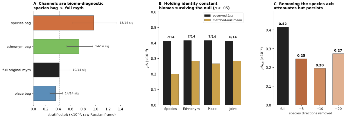
Figure 4. The alignment on the original, un-anonymised myths is not reducible to identity naming. All panels use the within-iconic-taxon stratified \Delta in the raw-Russian frame against iNaturalist images. Panel A : mean \Delta across the 14 biomes (with 95% bootstrap CI and the count of individually significant biomes) for the full original myth and three separately-measured identity baselines (species, place, ethnonym bags); the dashed line marks the full-myth level. A species-only bag is more biome-diagnostic than the full myth, and this survives stratification. Panel B : matched-permutation-null ladder — for each identity class, and for all three jointly, biome labels are shuffled only among motifs matched on that class’s identity-bag embedding (60 K-means blocks); bars give observed \mu\Delta_{full} (black) versus the matched-null mean (gold), annotated with the count of biomes whose observed \Delta exceeds the null at p < .05 . The place null is near-circular because biome is derived from the region metadata. Panel C : independent embedding-space control — the top k species-subspace directions are projected out of the full-myth embeddings and the stratified \Delta recomputed ( k = 5, 10, 20 ); \mu\Delta attenuates but stays positive and significant in the majority of biomes.
