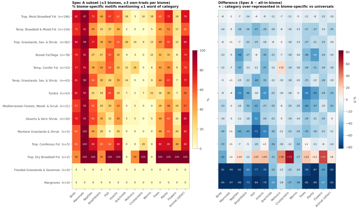
Figure 14. Ecological composition per biome (Spec A subset). Left: for each WWF biome (rows) and each of 14 taxonomic and botanical categories (columns), the cell shows the percentage of Spec A motifs (motifs touching \leq 3 biomes, \geq 3 own-traditions in that biome, the same selection that drives the headline result) whose raw Russian abstract mentions at least one species or plant of that category, before anonymisation. Right: difference (Spec A minus all-in-biome). Positive cells mark categories over-represented in biome-specific motifs relative to the universal-dominated full pool, revealing the ecological fingerprint that the species-hypernymisation layer subsequently removes. The all-motifs version of the heatmap is dominated by universal motifs and therefore uniformly red across biomes; we omit it here and release the underlying counts in the data drop.
