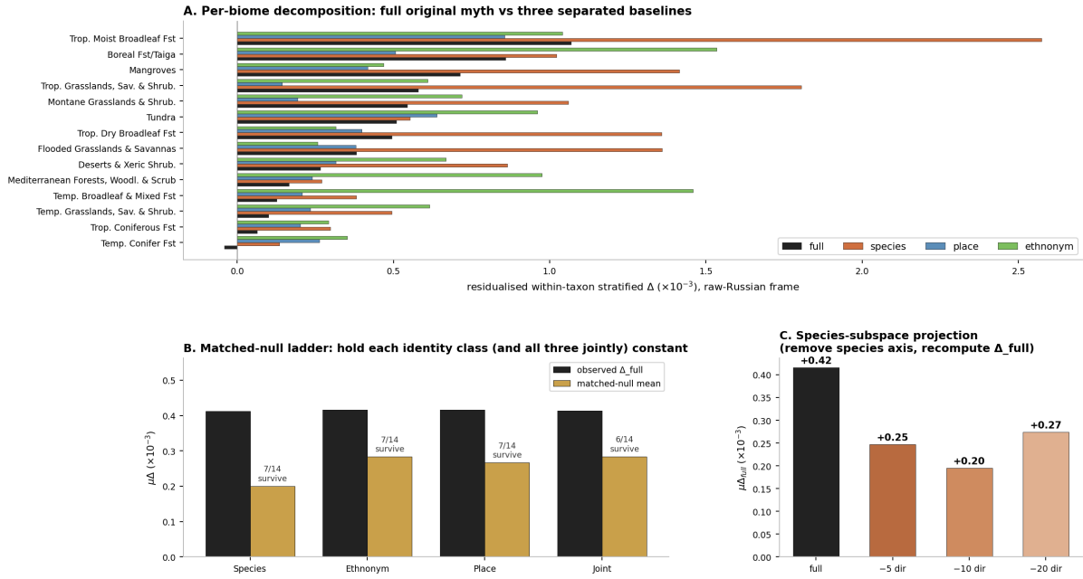
Figure 4. The alignment on the original, un-anonymised myths is not reducible to identity naming. All panels use the within-iconic-taxon stratified \Delta in the raw-Russian frame against iNaturalist images. Panel A : per-biome decomposition of the full original myth and three separately-measured identity baselines (species, place, ethnonym bags). A species-only bag is more biome-diagnostic than the full myth, and this survives stratification. Panel B : matched-permutation-null ladder — for each identity class, and for all three jointly, biome labels are shuffled only among motifs matched on that class’s identity-bag embedding (60 K-means blocks); bars give observed \mu\Delta_{full} (black) versus the matched-null mean (gold), annotated with the count of biomes whose observed \Delta exceeds the null at p < .05 . The place null is near-circular because biome is derived from the region metadata. Panel C : independent embedding-space control — the top k species-subspace directions are projected out of the full-myth embeddings and the stratified \Delta recomputed ( k = 5, 10, 20 ); \mu\Delta attenuates but stays positive and significant in the majority of biomes.
