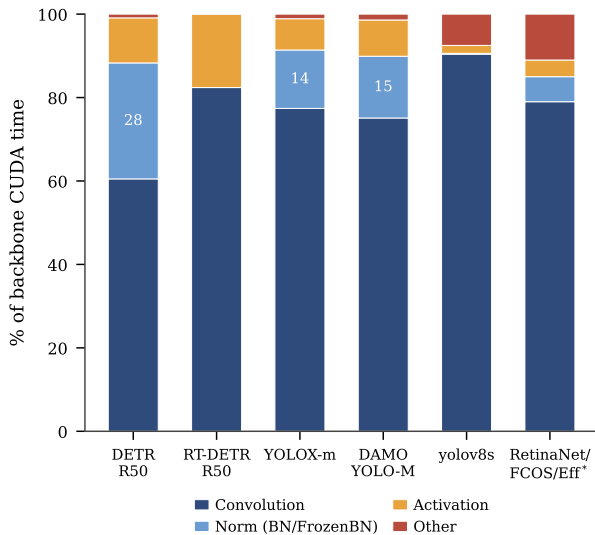
Figure 2: Backbone time by operation type (share of backbone CUDA time) for one representative model per family. Convolution dominates everywhere; the DETR family carries a large unfused FrozenBatchNorm block (28%) that the CNN detectors fold away. The last bar is the dense one-stage group (RetinaNet/FCOS/EfficientDet) as a whole-model 3-model aggregate.
