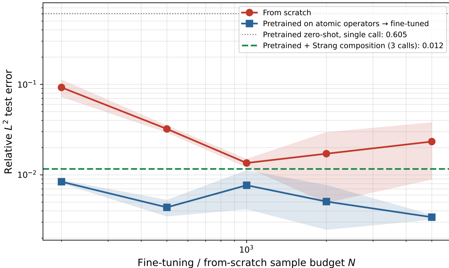
E2.b: Strang composition of a pretrained network in the commuting regime (target: constant-velocity advection-diffusion, s = 0 , 3 seeds)
