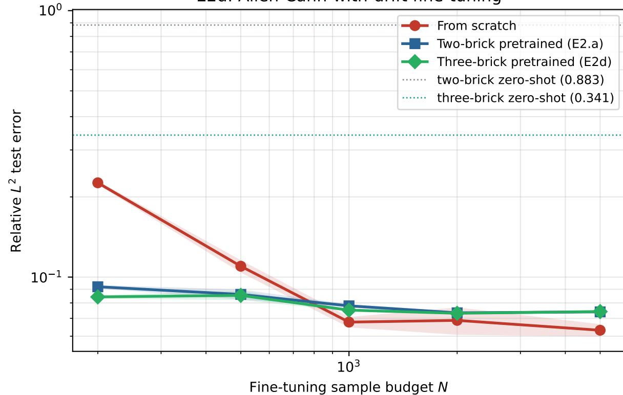
E2d: Allen-Cahn-with-drift fine-tuning
