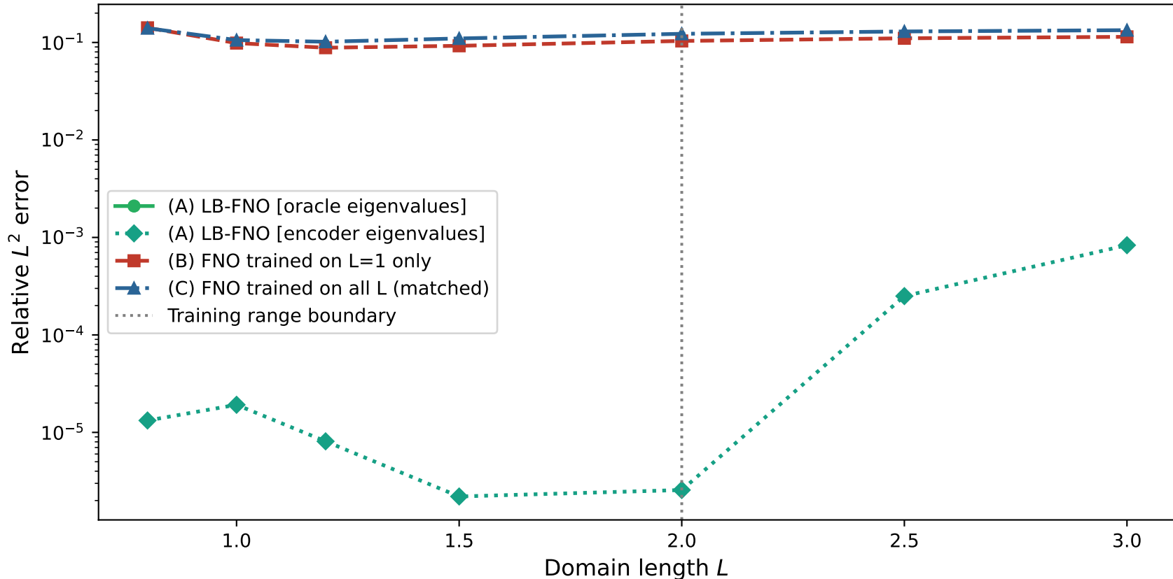
E3b: LB-FNO vs standard FNO across domain sizes (Phase A, Pillar 2)
