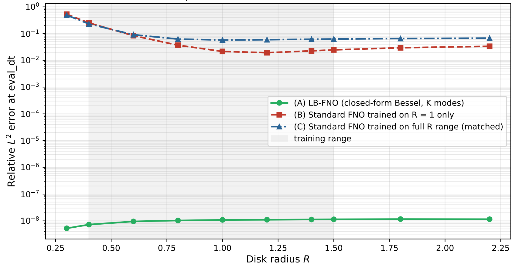
E3f: disk heat equation, LB-FNO vs standard 2D FNO (Phase A, Pillar 2)
