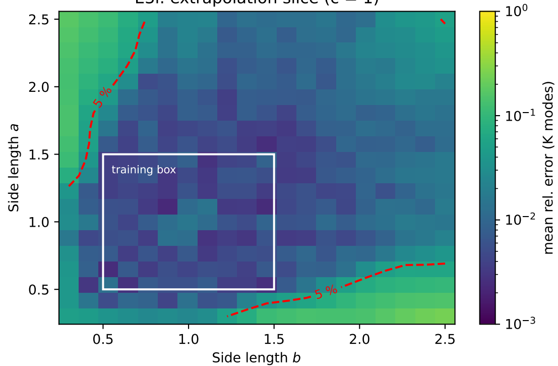
E3i: extrapolation slice (c = 1)
