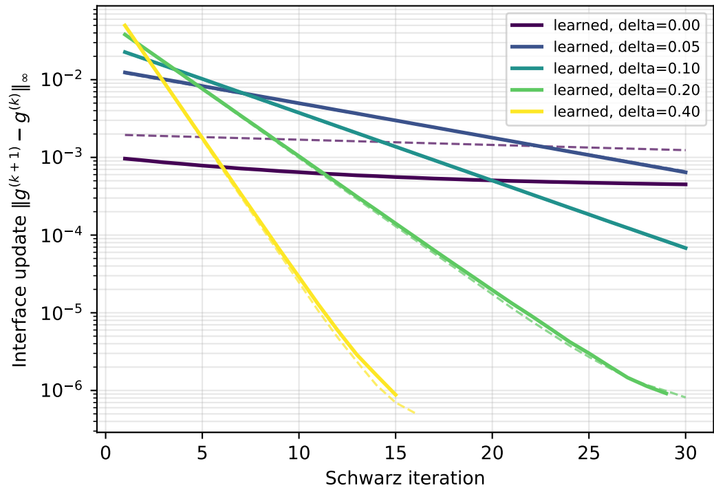
E4e: convergence curves (solid = learned, dashed = reference)
