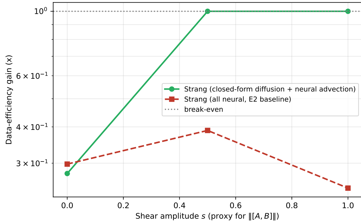
E5a: closed-form LB diffusion brick vs all-neural Strang
