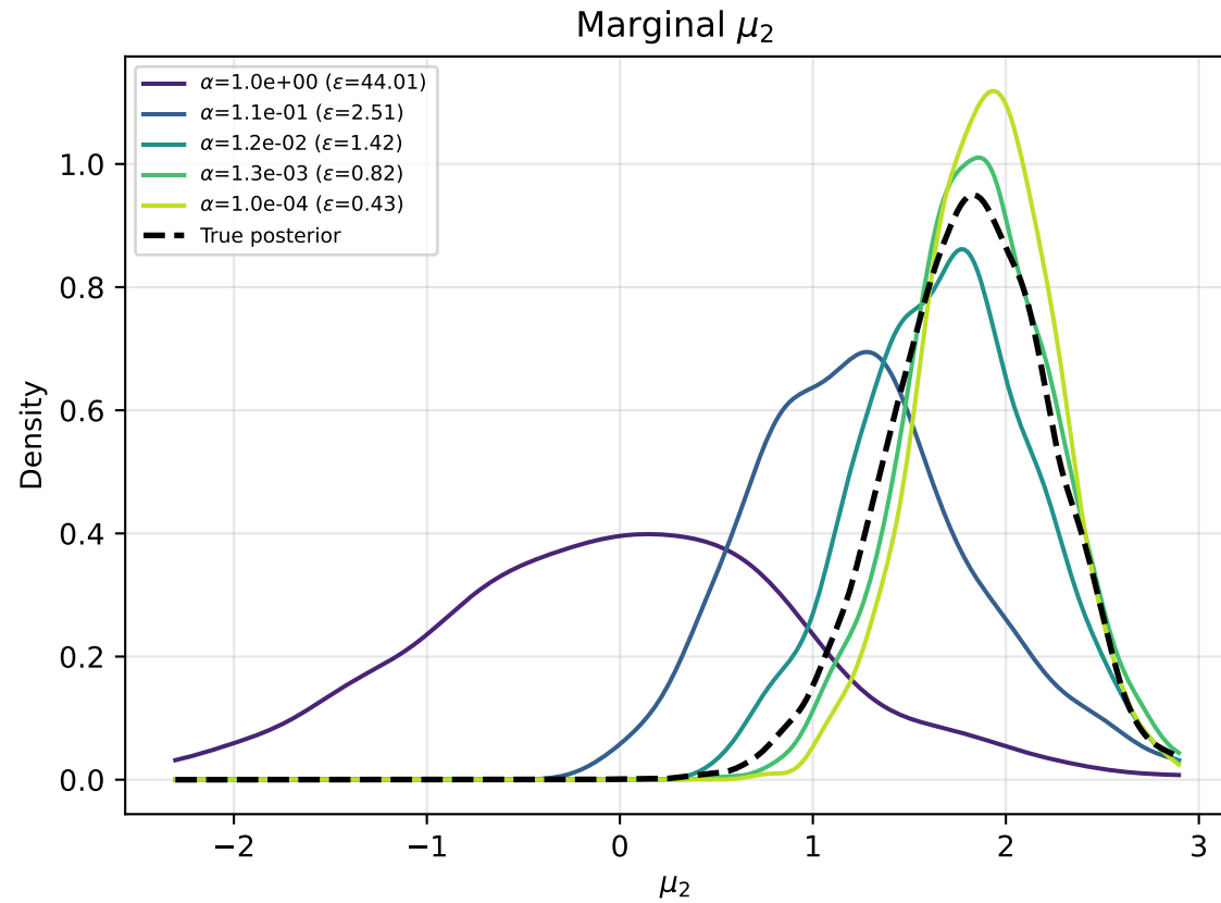
Marginal posteriors: ABC (summary stats) vs true — K=2
