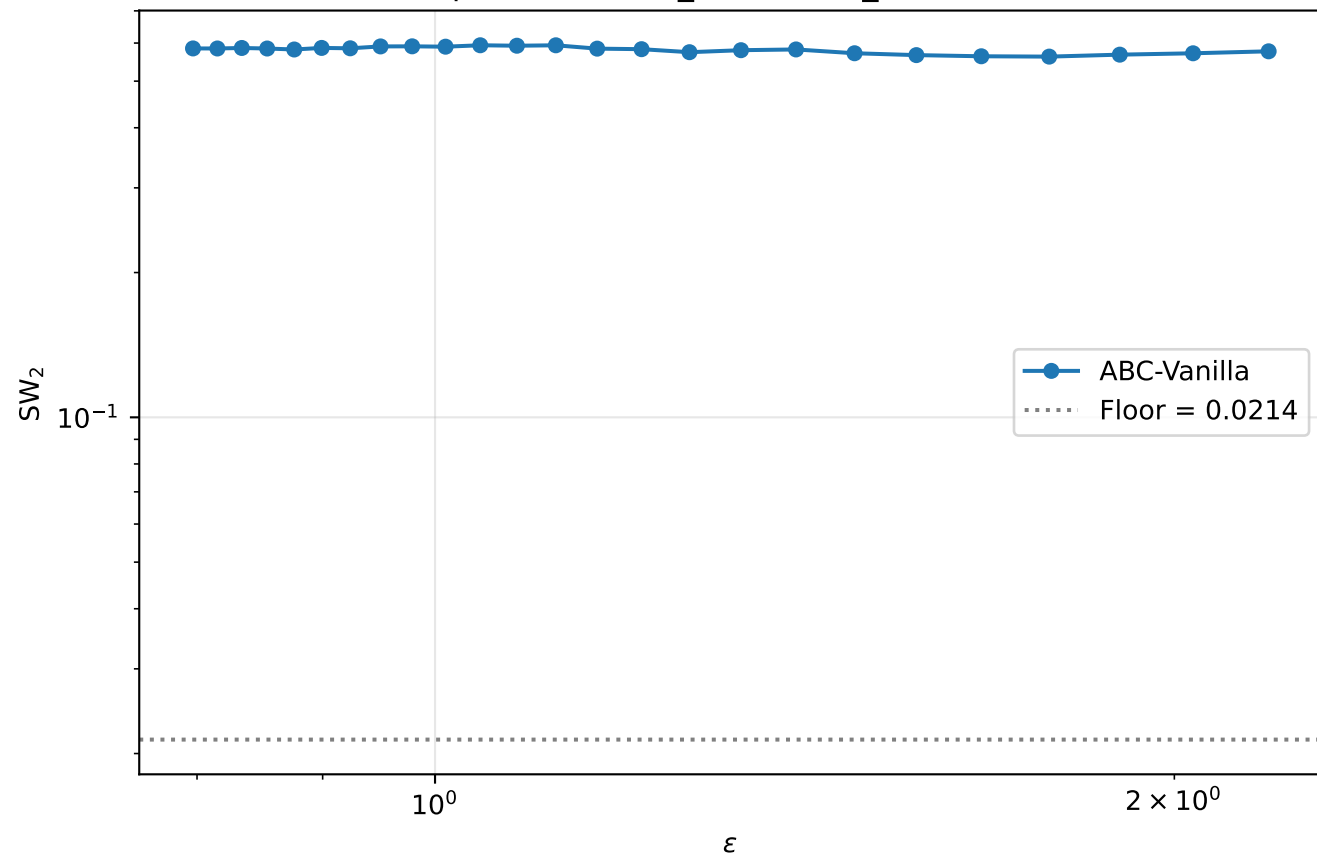
SW2 vs epsilon (K=2, n_obs=10, N_sim=10,000,000)
