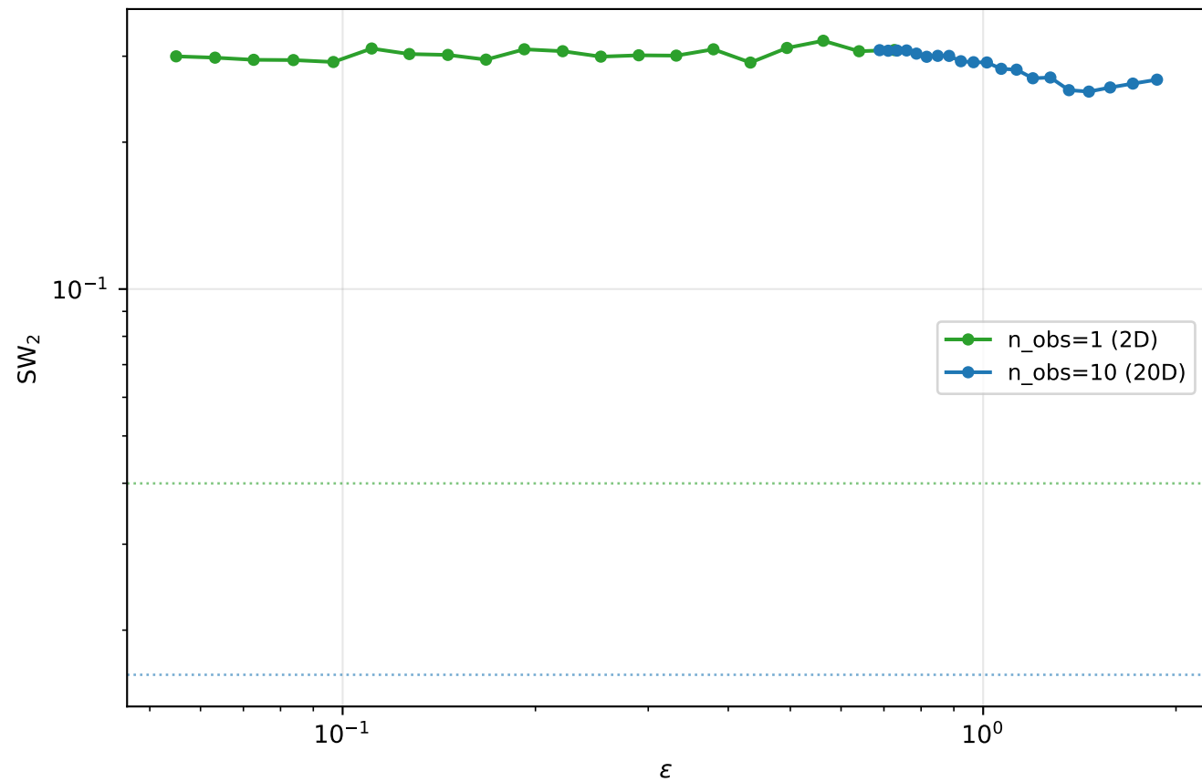
SW 2 vs \varepsilon — curse of dimensionality
