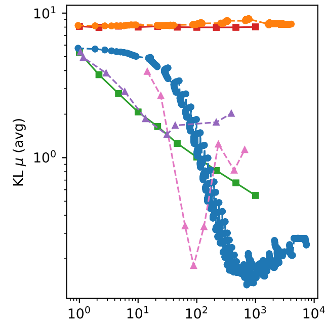
K=30, K_outliers=4
