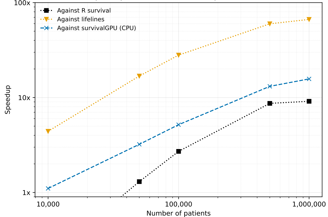
Speedup of the survivalGPU implementation
