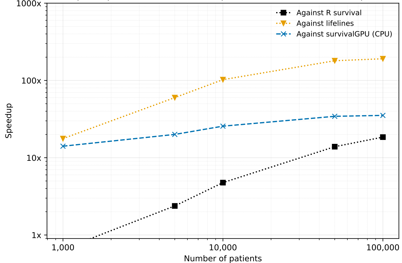
Speedup of the survivalGPU implementation (1000 bootstraps)
