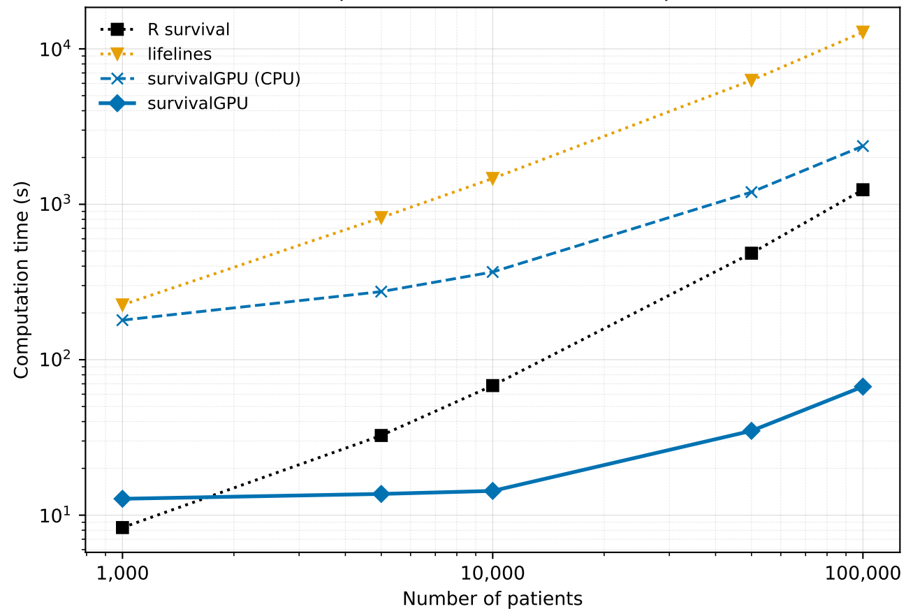
Computation time (1000 bootstraps)
