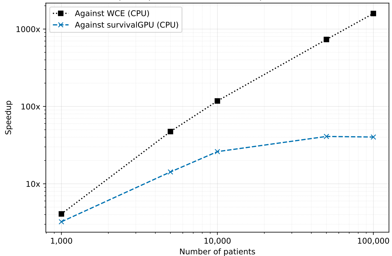
Speedup of the survivalGPU implementation
