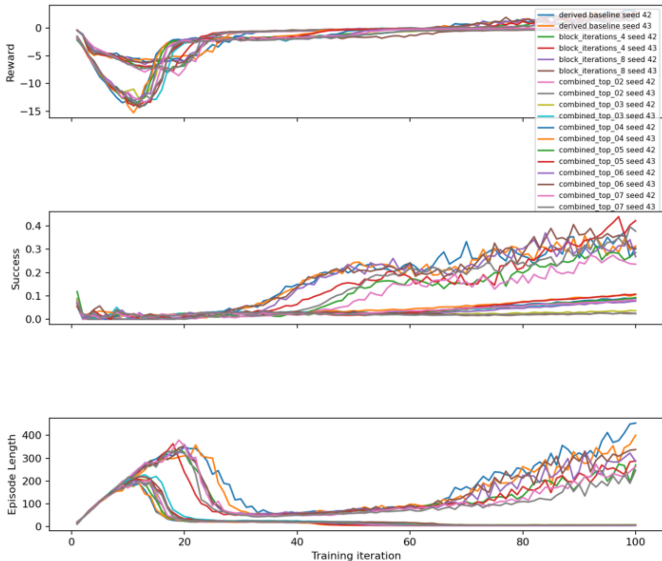
Stage 2 learning guardrails (including derived clean baseline)
