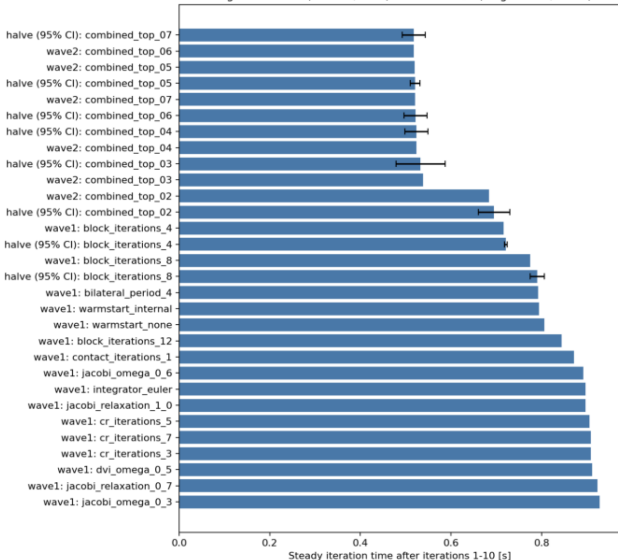
Stage-2 runtime (95% CI, n=2) and Wave 1/2 (single seed; no CI)
