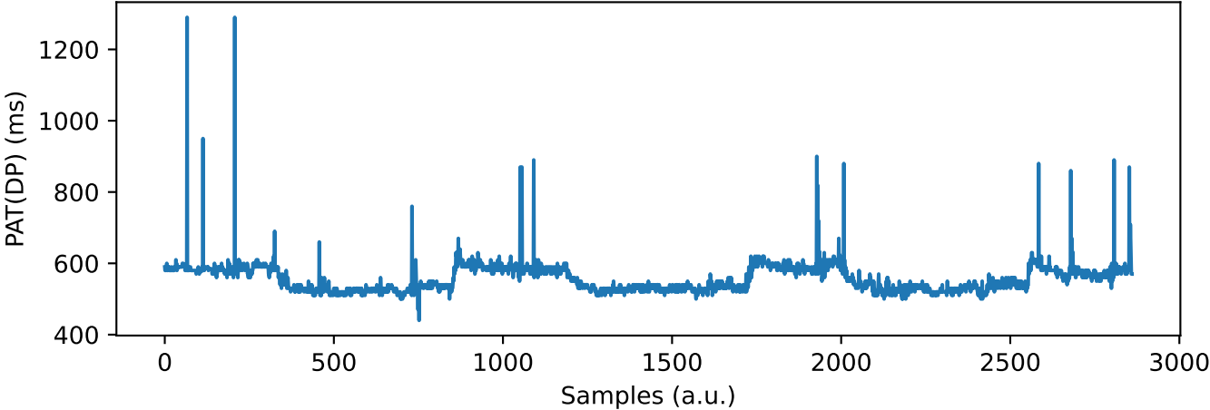
DBP_PAT(DP): \rho = -0.52 , SBP_PAT(DP): \rho = -0.01
