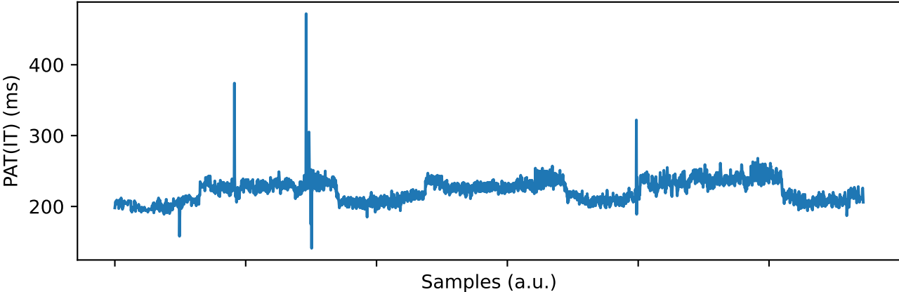
DBP_PAT(IT): \rho = 0.41 , SBP_PAT(IT): \rho = -0.01
