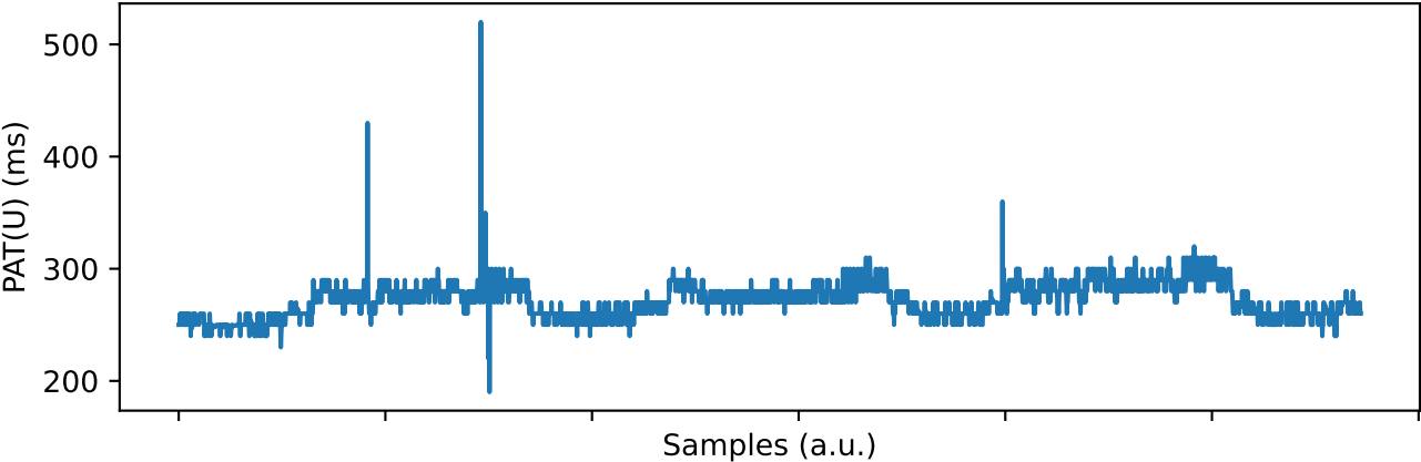
DBP_PAT(U): \rho = 0.4 , SBP_PAT(U): \rho = -0.01
