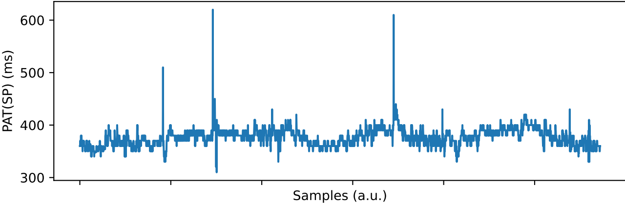
DBP_PAT(SP): \rho = 0.21 , SBP_PAT(SP): \rho = 0.07
