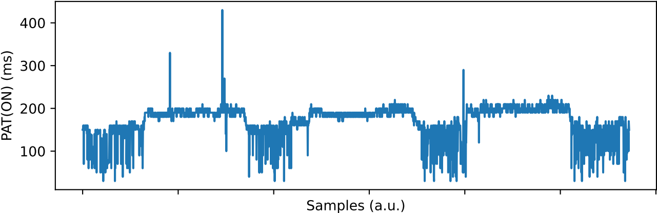
DBP_PAT(ON): \rho = 0.42 , SBP_PAT(ON): \rho = -0.02
