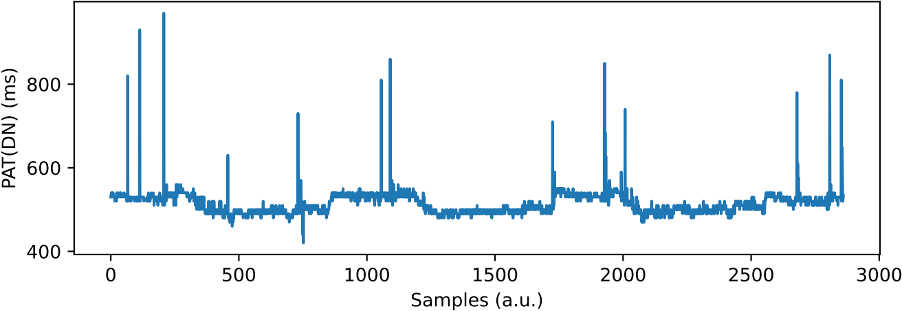
DBP_PAT(DN): \rho = -0.49 , SBP_PAT(DN): \rho = 0.0
