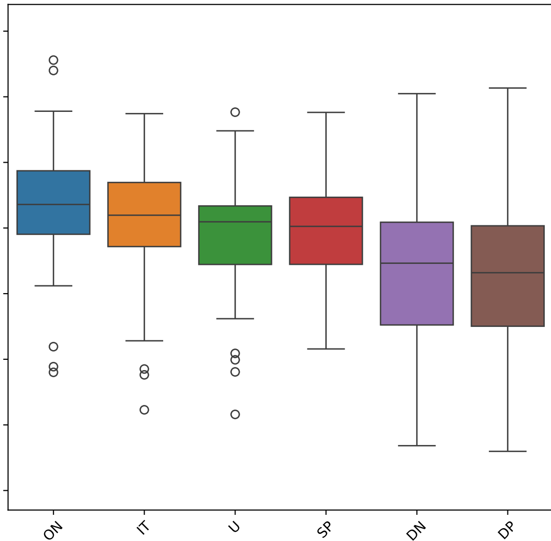
Spearman Correlation between PAT types and SBP
