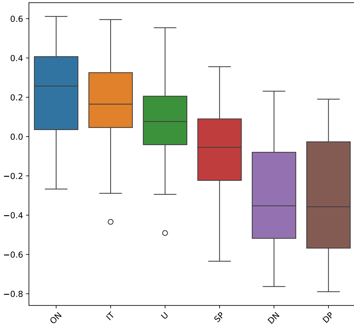
Spearman Correlation between PAT types and DBP
