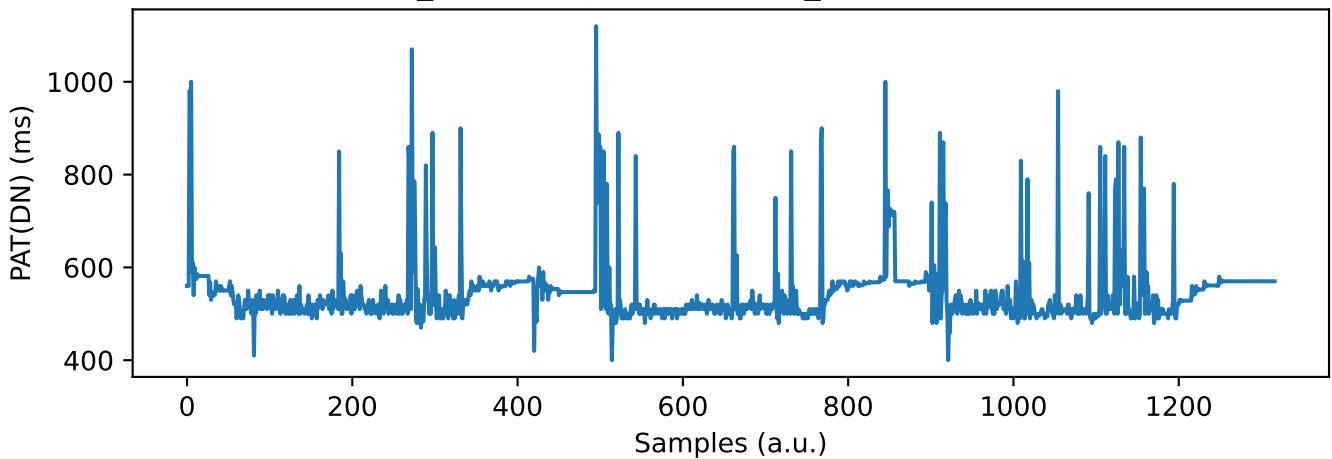
DBP_PAT(DN): \rho = 0.04 , SBP_PAT(DN): \rho = 0.09
