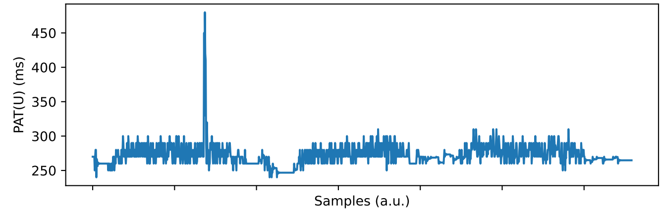
DBP_PAT(U): \rho = 0.01 , SBP_PAT(U): \rho = 0.03
