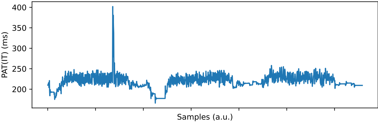
DBP_PAT(IT): \rho = 0.05 , SBP_PAT(IT): \rho = 0.03
