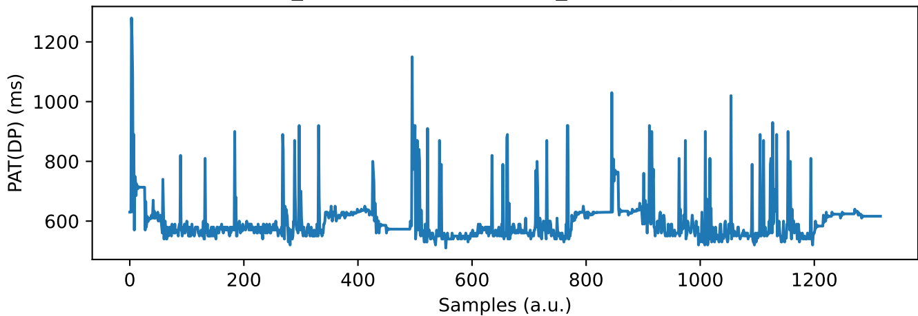
DBP_PAT(DP): \rho = 0.03 , SBP_PAT(DP): \rho = 0.09
