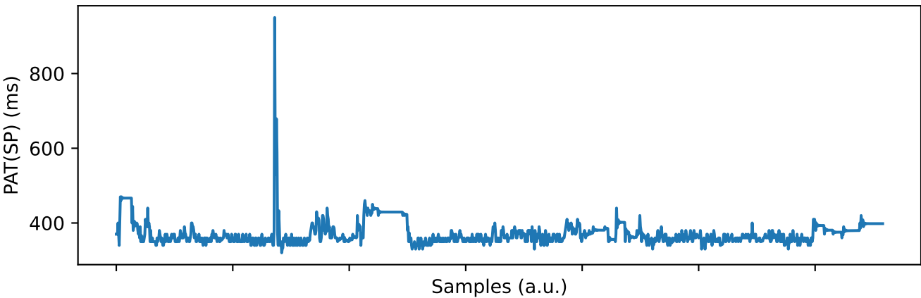
DBP_PAT(SP): \rho = -0.05 , SBP_PAT(SP): \rho = 0.04
