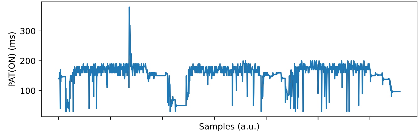
DBP_PAT(ON): \rho = 0.03 , SBP_PAT(ON): \rho = -0.01
