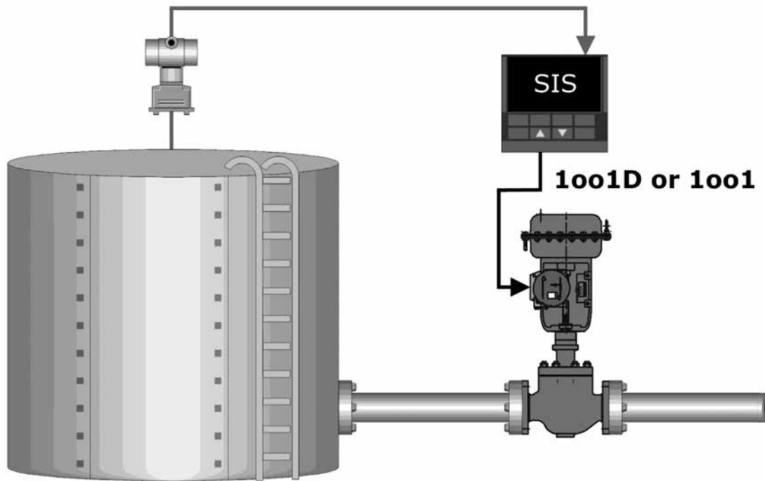
Figure 1. Schematical picture of safety loop. Final element is connected to safety system (SIS) via solenoid or safety valve controller (partial stroke device). This shows single channel final element subsystem with voting 1oo1D or 1oo1.
