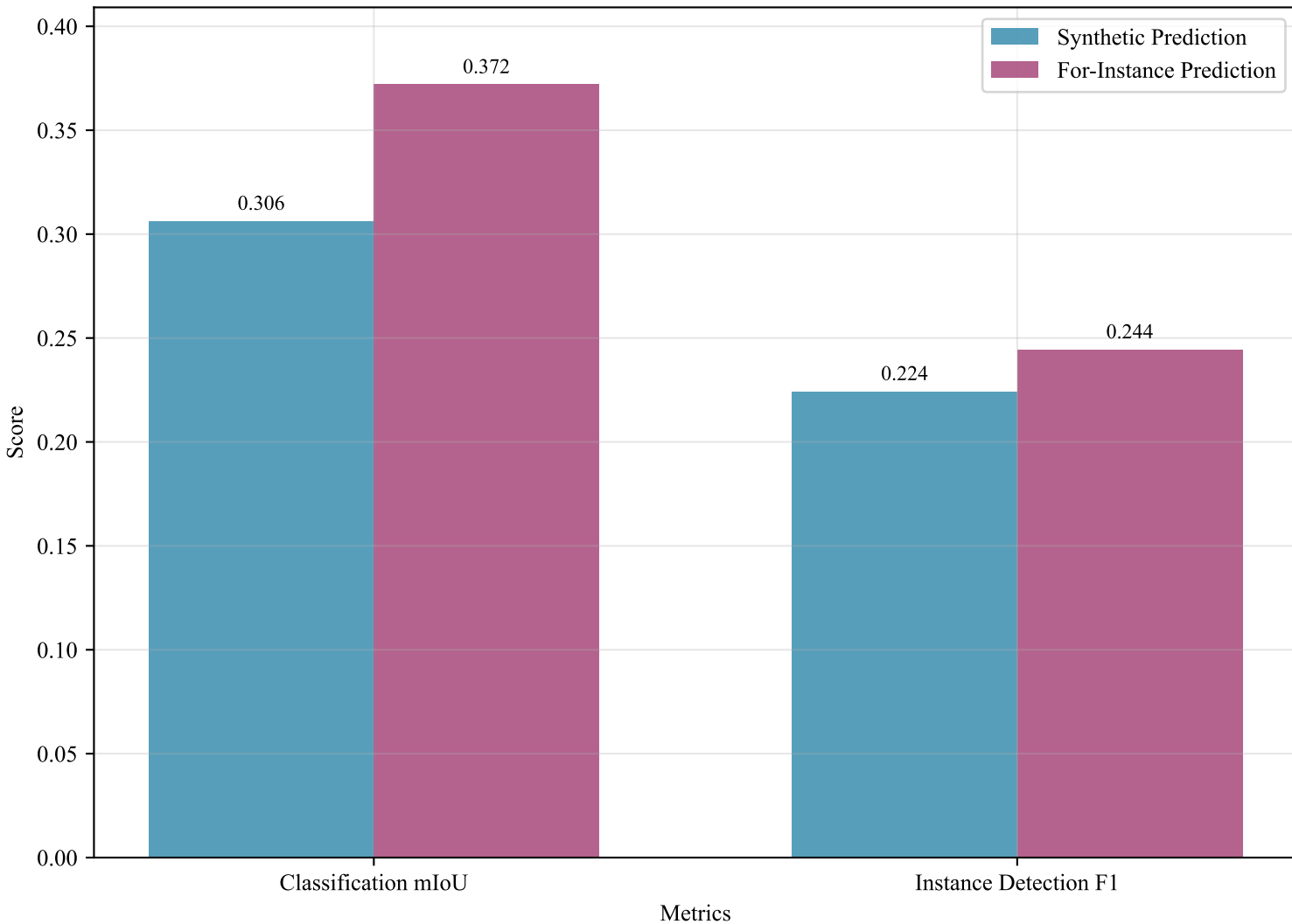
Overall Metrics Comparison
