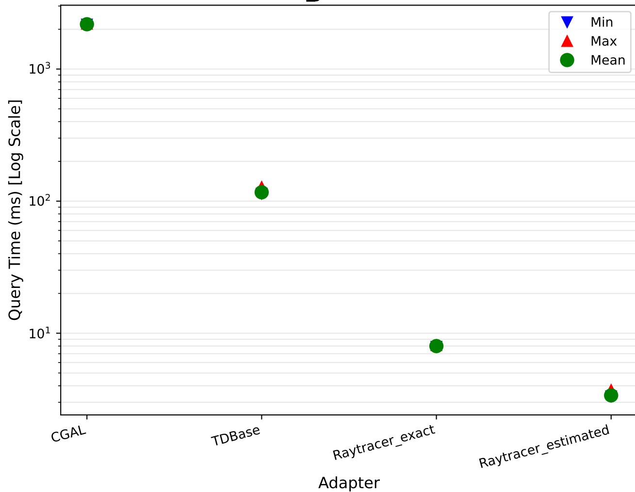
Min/Max/Mean Comparison nuclei_join (20 runs)
