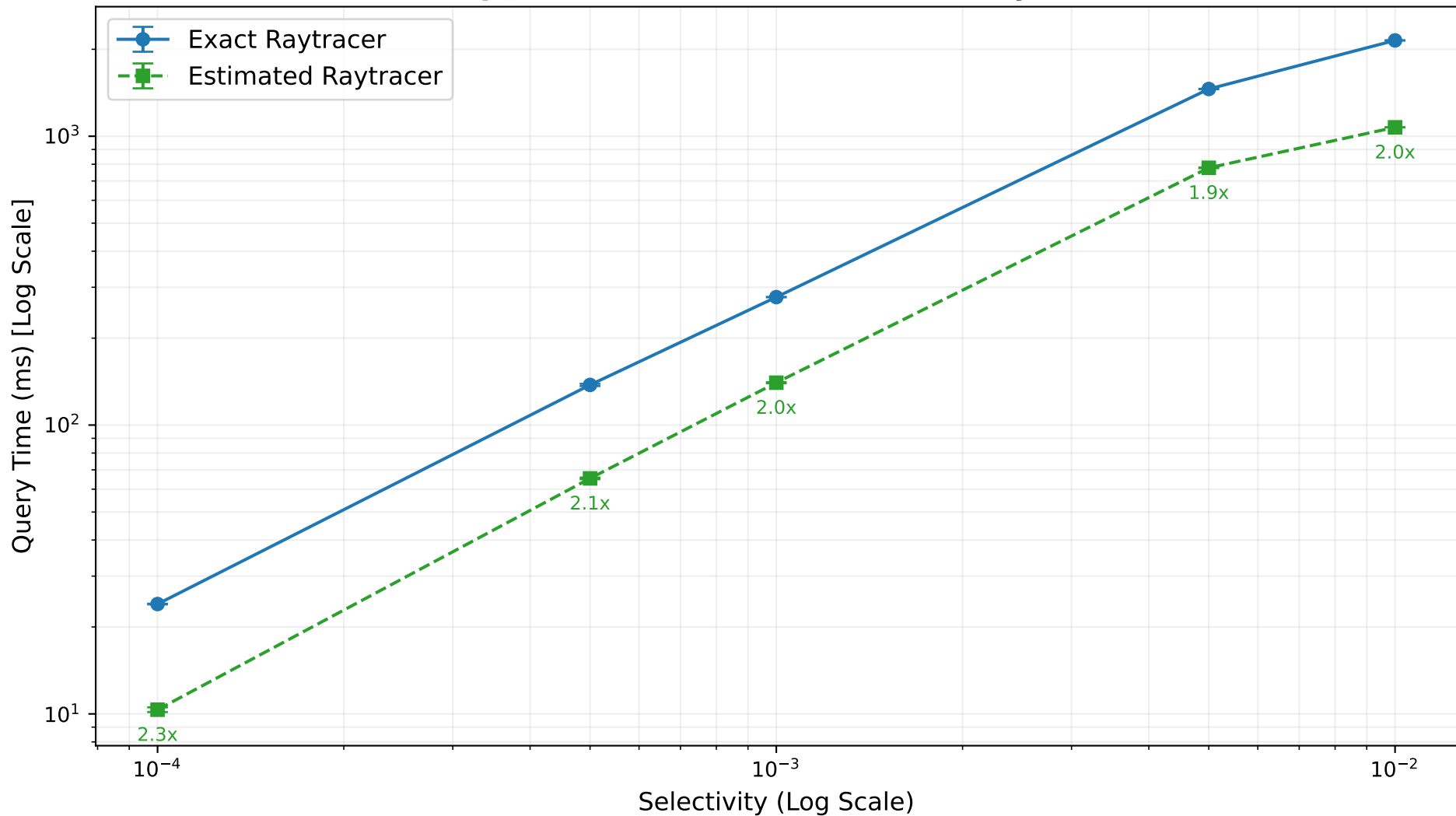
Mesh Overlap Join Performance vs. Selectivity (50000 cubes)
