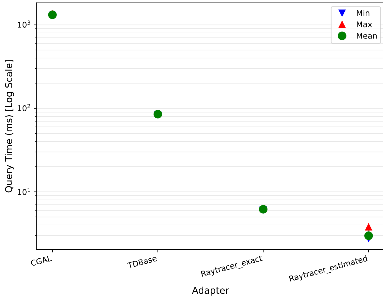
Min/Max/Mean Comparison medium (20 runs)
