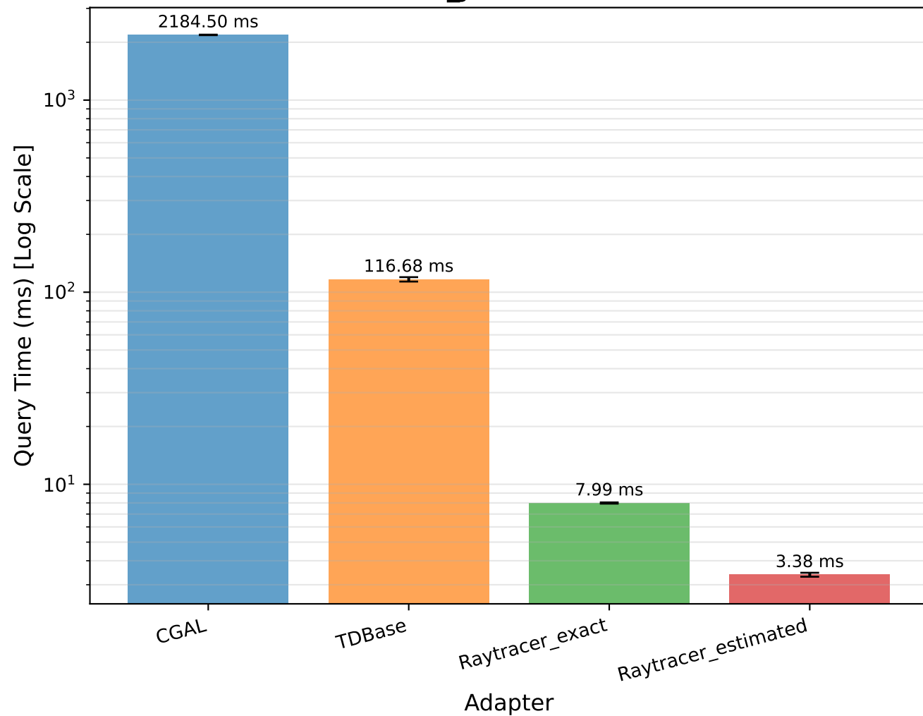
Mean Query Time with Std Dev nuclei_join (20 runs)
