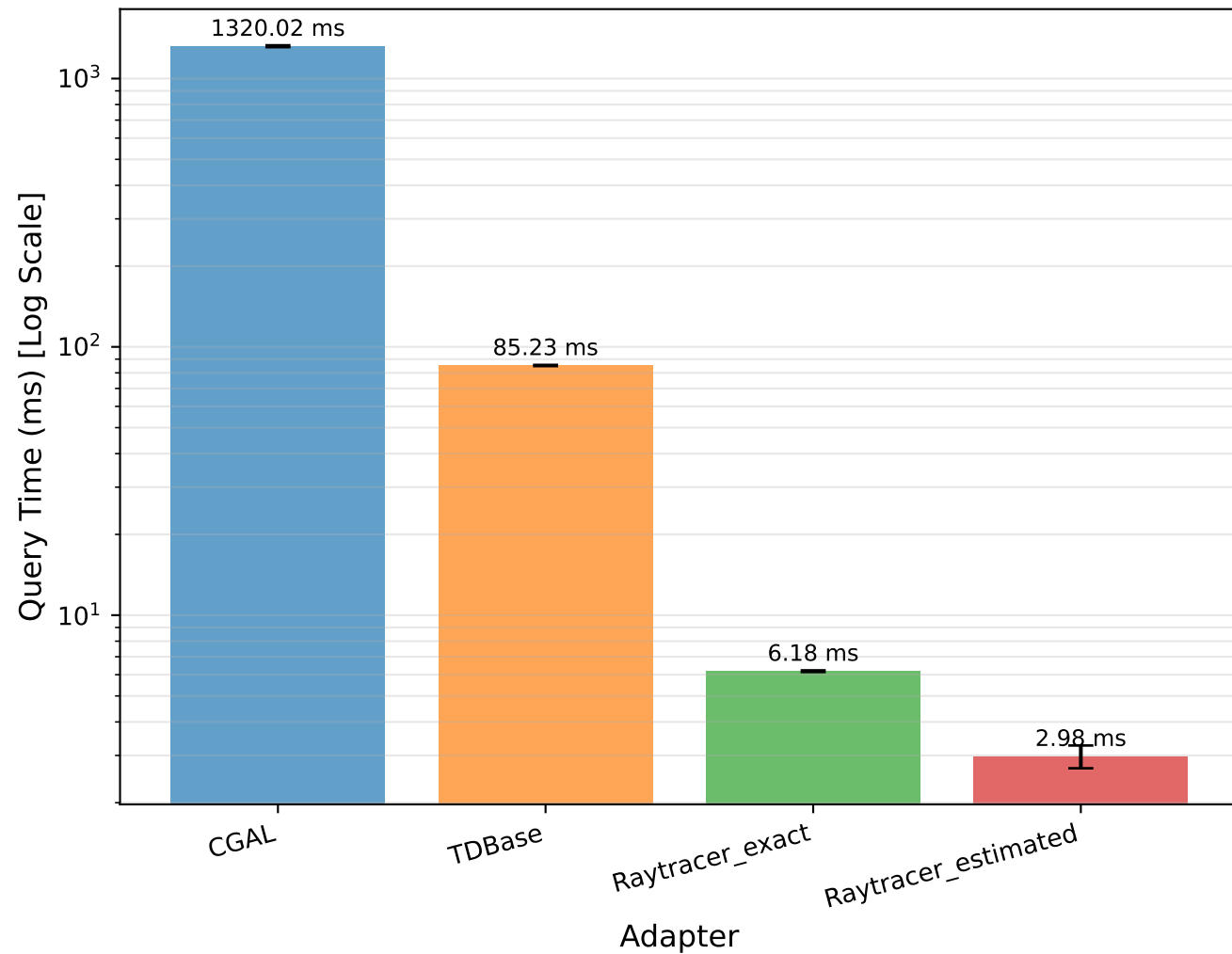
Mean Query Time with Std Dev medium (20 runs)
