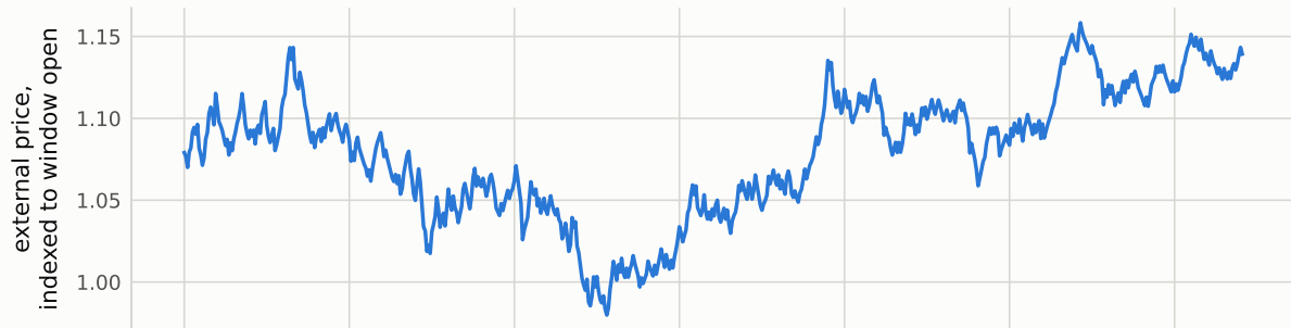
VolatilityHook
