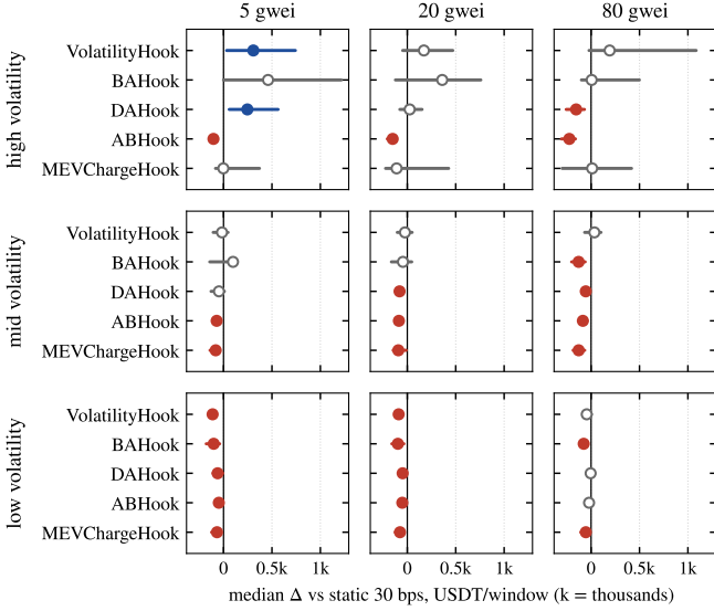
Fig. 4. The same decomposition at the informed-heavy point ( \kappa=0.1 , arbitrage 58% of volume): the storm-cheap-gas corner strengthens and changes owners.
