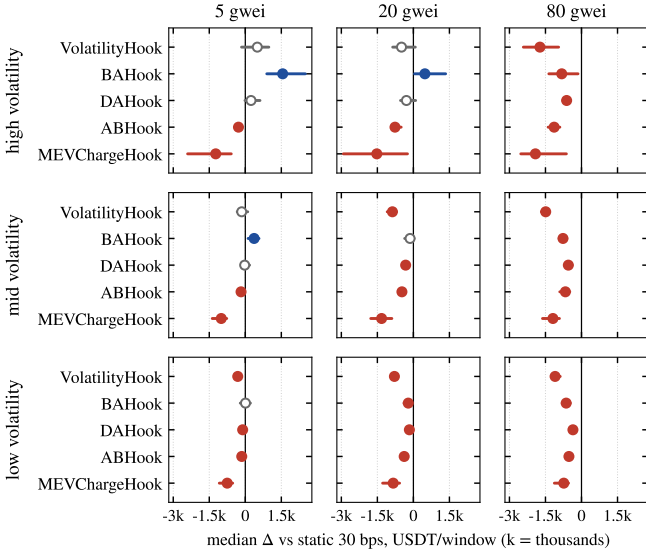
Fig. 3. Conditional structure at \kappa=1 : median paired advantage over the 30 bps baseline by volatility regime \times gas scenario (volatile pairs pooled, 48 windows per panel; filled marker = 95% CI excludes zero; blue wins, orange loses).
