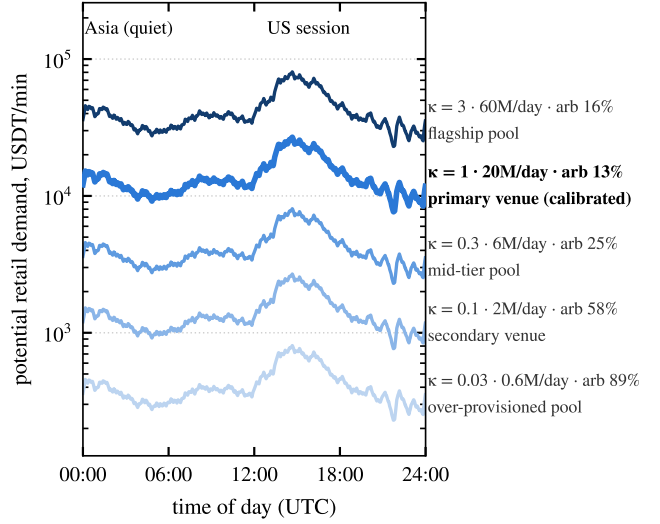
Fig. 1. Demand calibration, Eq. (5): the intraday shape \hat{s}(c) is measured (median 2024 day of the pair’s Binance legs); the single knob \kappa scales its height, and the height sets the arbitrage share of volume the experiment measures.
