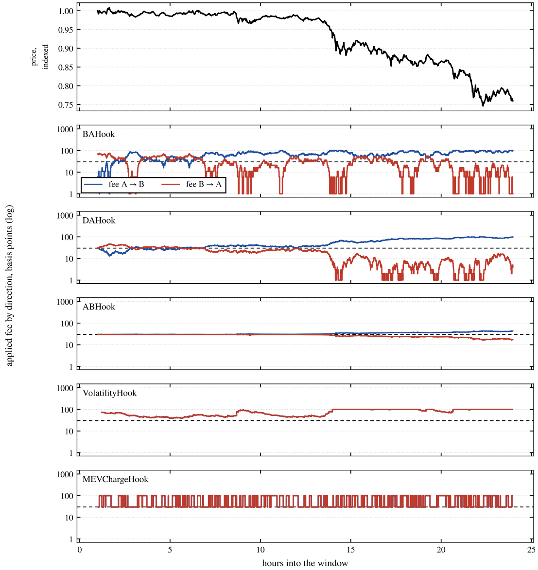
Fig. 2. What each hook actually charged through one high-volatility ETH/SHIB day (2024-03-01, 20 gwei, \kappa=1 ; log fee axis shared across panels; dashed = the 30 bps baseline). Each mark is the fee of an executed swap, held forward; for the directional hooks the two directions’ fees interleave as swap direction alternates, which produces the sawtooth.
