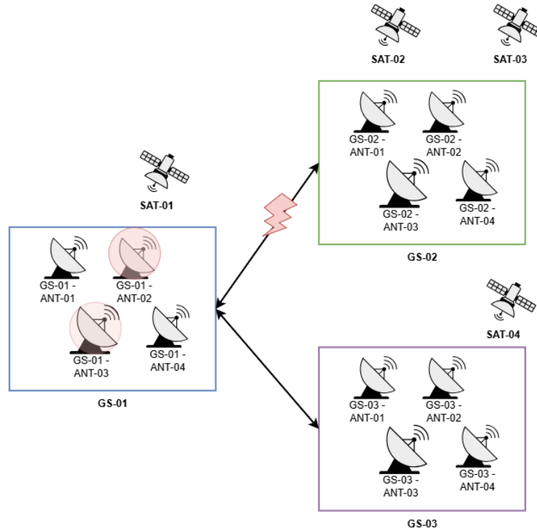
Figure 5.1: Overview of the evaluation scenario: there are 3 ground segment stations GS-01, GS-02, and GS-03, each with 4 antennas, and 4 satellites SAT-01, SAT-02, SAT-03, and SAT-04. GS-01 is connected to both GS-02 and GS-03 through inter-station network links. The link between GS-01 and GS-02 is degraded, while the link between GS-01 and GS-03 is operational but exhibits increased latency. GS-01/ANT-02 is unavailable, while GS-01/ANT-03 is degraded. The remaining antennas of GS-01 are operational, while GS-02 and GS-03 are nominal at station level. The ANT positioning is close to the respective ground stations.
