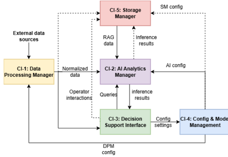
Figure 3.1: The Funes high level software architecture is composed of 5 Configuration Items. The data flows from external subsystems to the Data Processing Manager (DPM) module which will turn them into an internal standard data representation after performing cleaning and validation. The data is then fed to the Storage Manager (SM) for being stored and to the AI Analytics for AI processing. The user utilizes the system through the Decision Support Interface (DSI). The Config & model management module is responsible for the system configuration and AI control.
