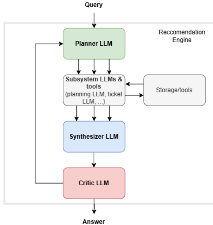
Figure 4.3: Multi-agent reasoning workflow of the AI Manager, showing the iterative interaction between the Planner, tool-based evidence retrieval, Synthesizer, and Critic agents.
