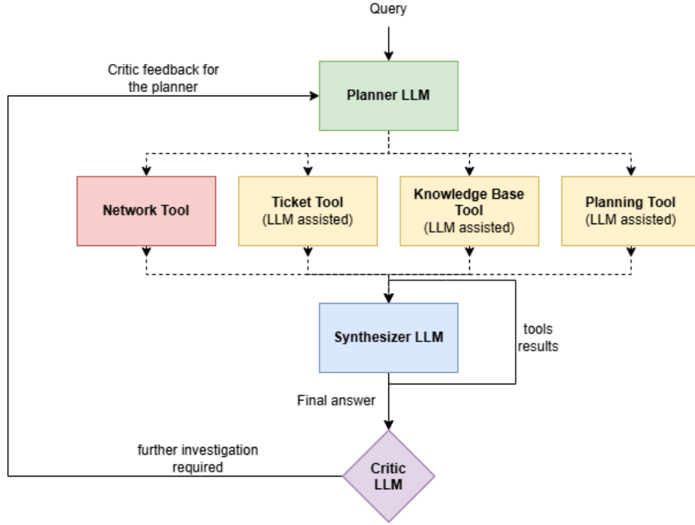
Figure 4.4: This figure summarizes the workflow of the different agents of the system. The mission manager query is passed to the planner agent that decides what tools and agents have to be called to answer. The results are then passed to the Synthesizer that will provide a final answer. The synthesizer’s response and the tools results are then passed to the critic that will determine if other tools are necessary for a more complete response. If so the critic will generate a feedback that is given to the planner for a plan refinement and another tool calling, only the new tools are going to be called if the inputs for the others are unchanged.
