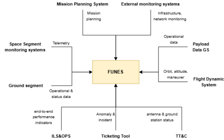
Figure 3.2: The funes system context diagram shows the main external systems that interact with the FUNES system. The data flows continuously from the external systems to FUNES and then to the user through the decision support interface, showed in Fig. 3.3.
