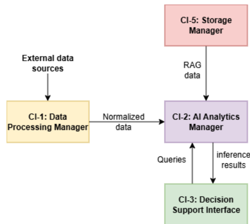
Figure 3.5: Conversational data flow for AI-assisted operator investigation, showing query submission, historical data retrieval, RAG-based analysis, and interactive response generation.
