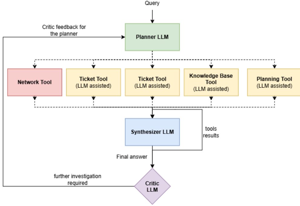
Figure 4.4: This figure summarizes the workflow of the different agents of the system. The mission manager query is passed to the planner agent that decides what tools and agents have to be called to answer. The results are then passed to the Synthesizer that will provide a final answer. The synthesizer’s response and the tools results are then passed to the critic that will determine if other tools are necessary for a more complete response. If so the critic will generate a feedback that is given to the planner for a plan refinement and another tool calling, only the new tools are going to be called if the inputs for the others are unchanged.
