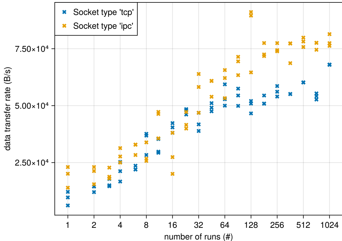
Test graph communication, sent data packet size = 1 B, 7 transfers
